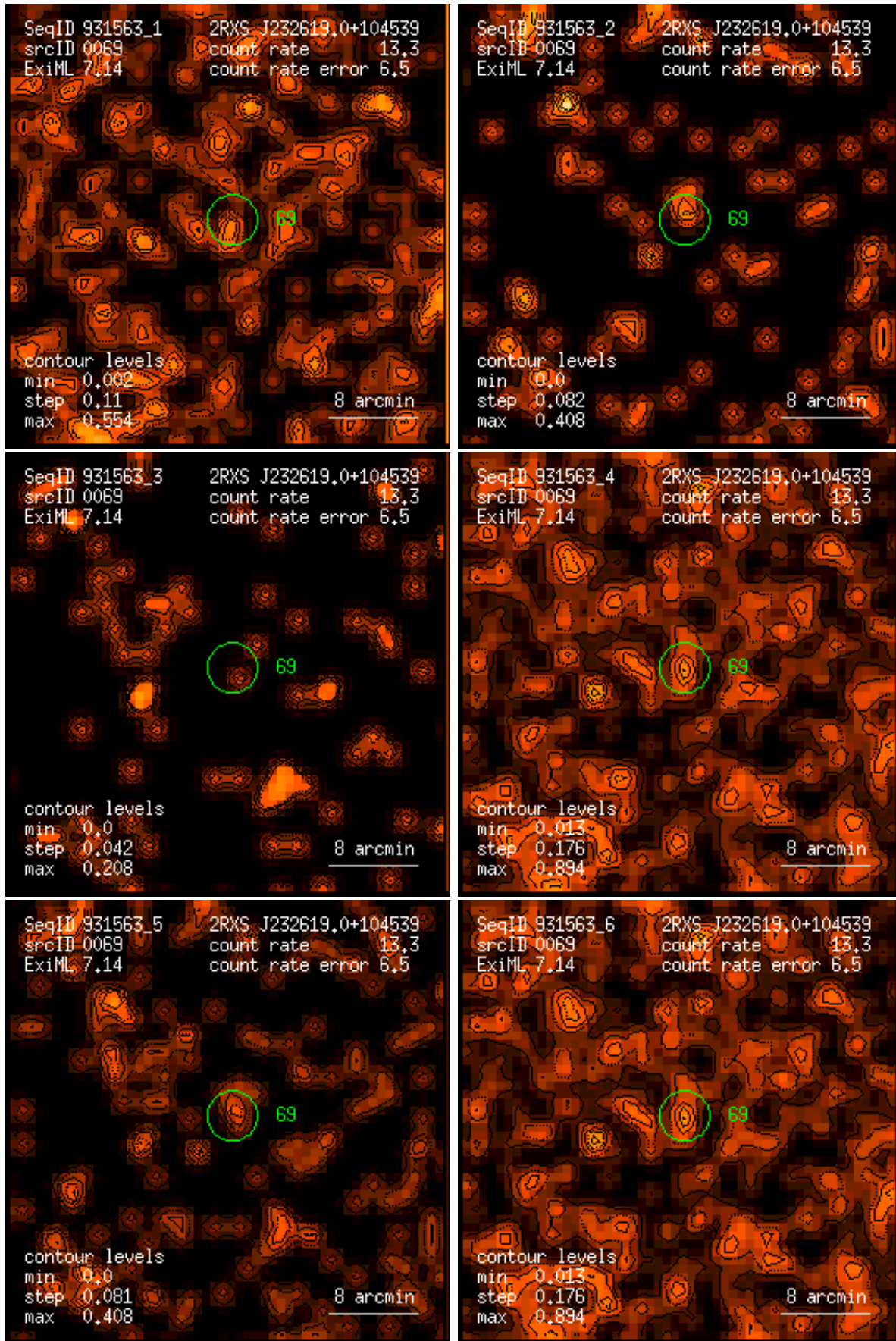
Figure 69: RASS 931563: detection 0069: band rate images, Gaussian filter: (1) PSPC channels 11 – 41, (2) 52 – 90, (3) 91 – 201, (4) 11 – 235, (5) 52 – 201, (6) 11 – 201. Broad band rates in counts/ks. Band rate contour levels in counts/ks/arcmin 2 .
