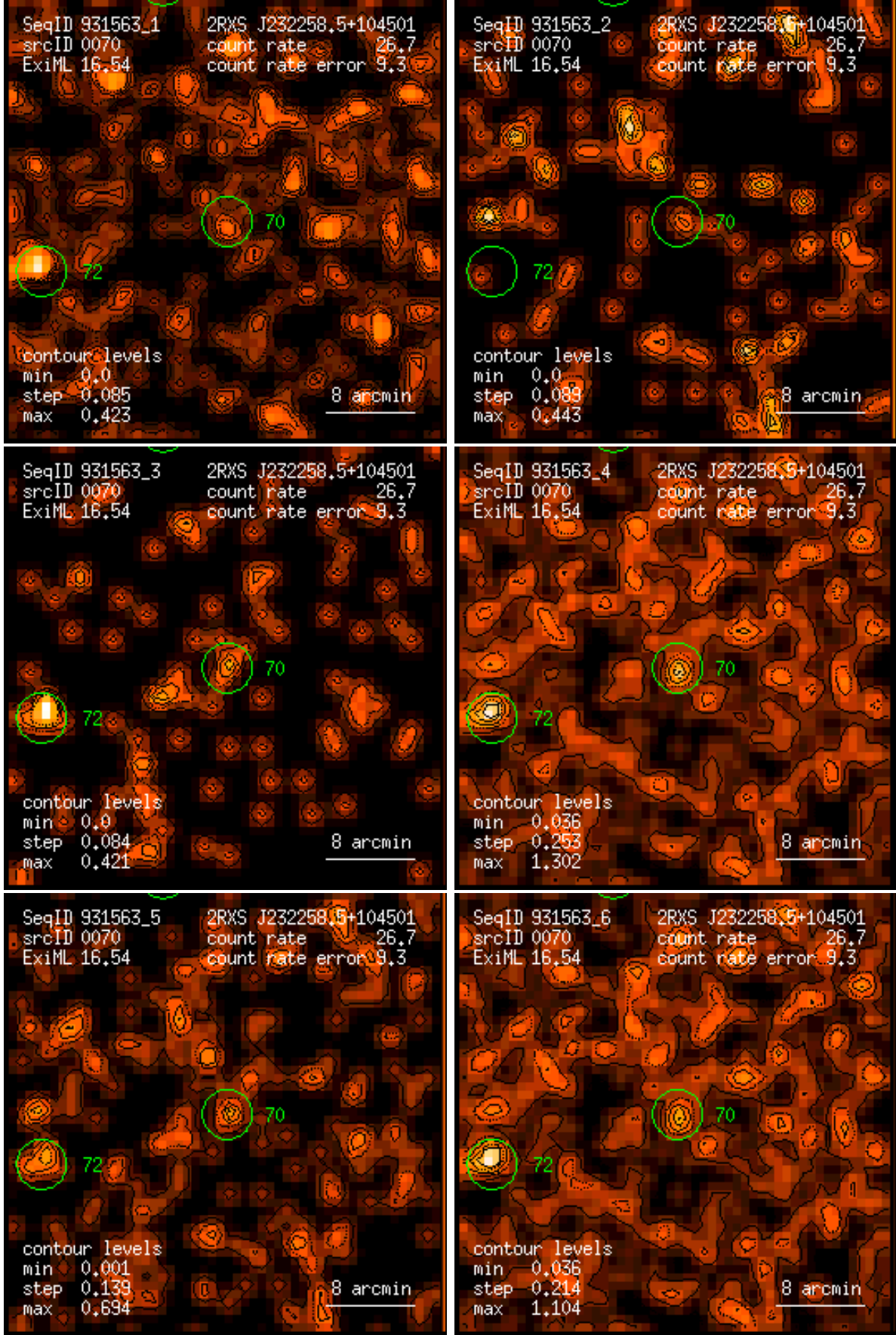
Figure 70: RASS 931563: detection 0070: band rate images, Gaussian filter: (1) PSPC channels 11 – 41, (2) 52 – 90, (3) 91 – 201, (4) 11 – 235, (5) 52 – 201, (6) 11 – 201. Broad band rates in counts/ks. Band rate contour levels in counts/ks/arcmin 2 .
