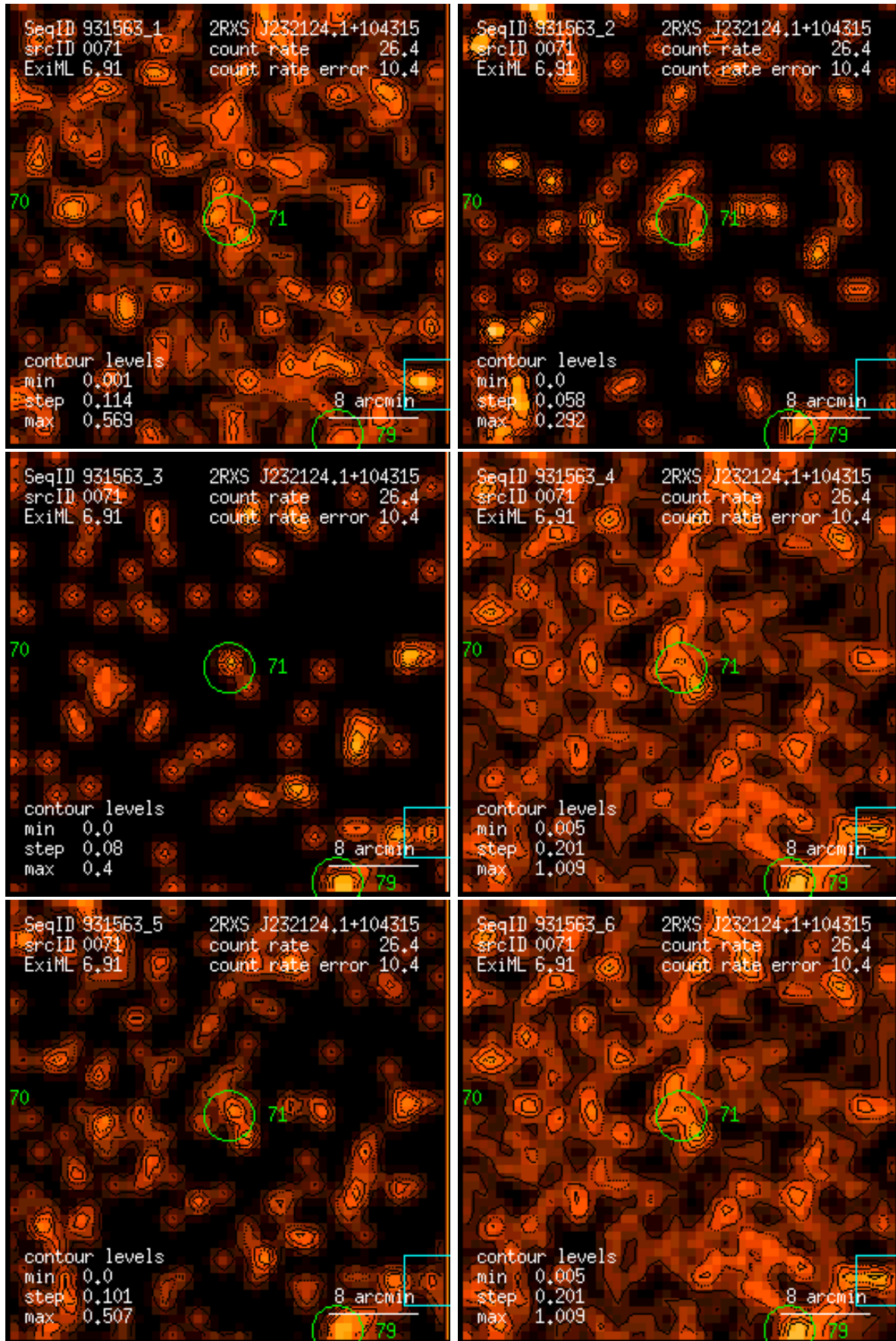
Figure 71: RASS 931563: detection 0071: band rate images, Gaussian filter: (1) PSPC channels 11 – 41, (2) 52 – 90, (3) 91 – 201, (4) 11 – 235, (5) 52 – 201, (6) 11 – 201. Broad band rates in counts/ks. Band rate contour levels in counts/ks/arcmin 2 .
