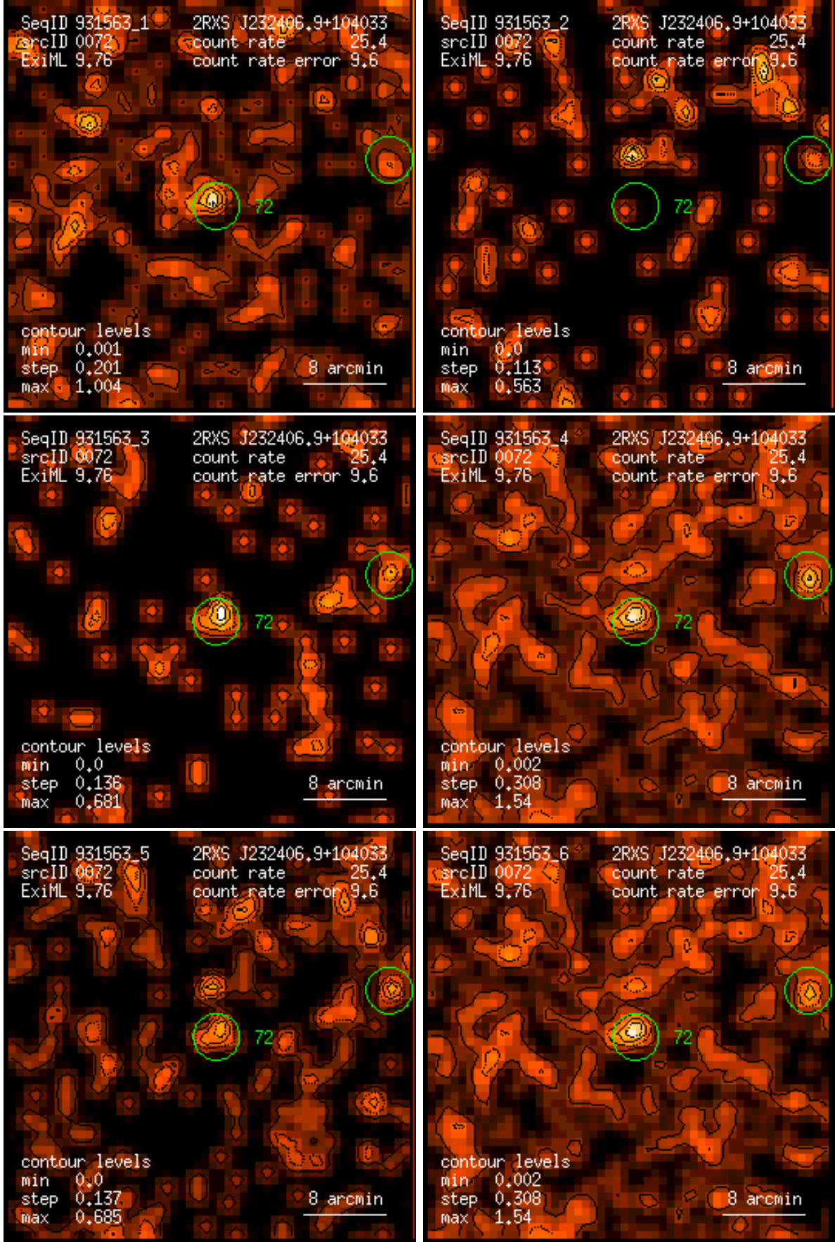
Figure 72: RASS 931563: detection 0072: band rate images, Gaussian filter: (1) PSPC channels 11 – 41, (2) 52 – 90, (3) 91 – 201, (4) 11 – 235, (5) 52 – 201, (6) 11 – 201. Broad band rates in counts/ks. Band rate contour levels in counts/ks/arcmin 2 .
