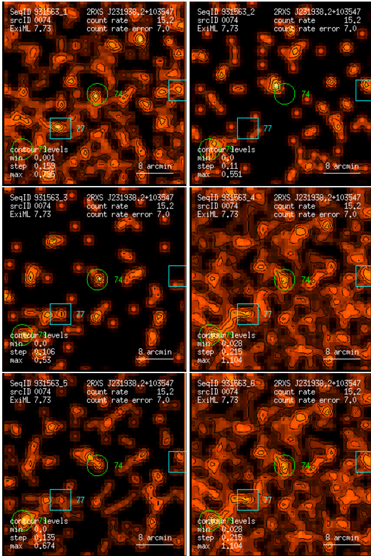
Figure 74: RASS 931563: detection 0074: band rate images, Gaussian filter: (1) PSPC channels 11 – 41, (2) 52 – 90, (3) 91 – 201, (4) 11 – 235, (5) 52 – 201, (6) 11 – 201. Broad band rates in counts/ks. Band rate contour levels in counts/ks/arcmin 2 .
