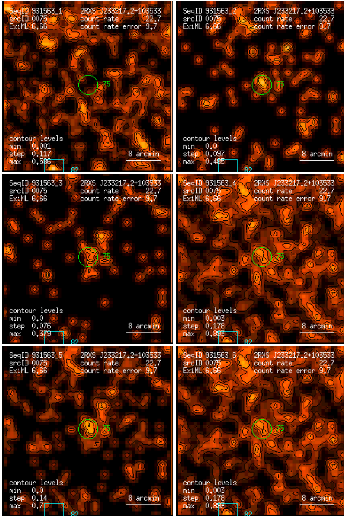
Figure 75: RASS 931563: detection 0075: band rate images, Gaussian filter: (1) PSPC channels 11 – 41, (2) 52 – 90, (3) 91 – 201, (4) 11 – 235, (5) 52 – 201, (6) 11 – 201. Broad band rates in counts/ks. Band rate contour levels in counts/ks/arcmin 2 .
