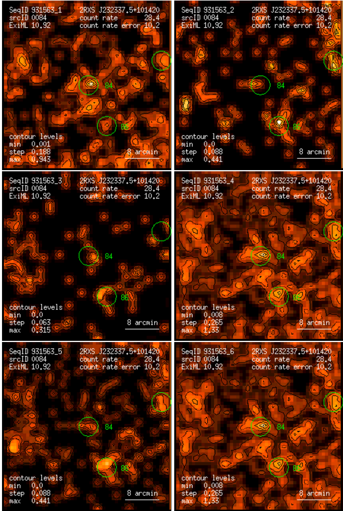
Figure 84: RASS 931563: detection 0084: band rate images, Gaussian filter: (1) PSPC channels 11 – 41, (2) 52 – 90, (3) 91 – 201, (4) 11 – 235, (5) 52 – 201, (6) 11 – 201. Broad band rates in counts/ks. Band rate contour levels in counts/ks/arcmin 2 .
