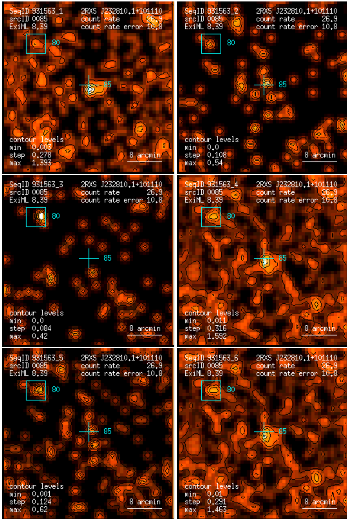
Figure 85: RASS 931563: detection 0085: band rate images, Gaussian filter: (1) PSPC channels 11 – 41, (2) 52 – 90, (3) 91 – 201, (4) 11 – 235, (5) 52 – 201, (6) 11 – 201. Broad band rates in counts/ks. Band rate contour levels in counts/ks/arcmin 2 .
