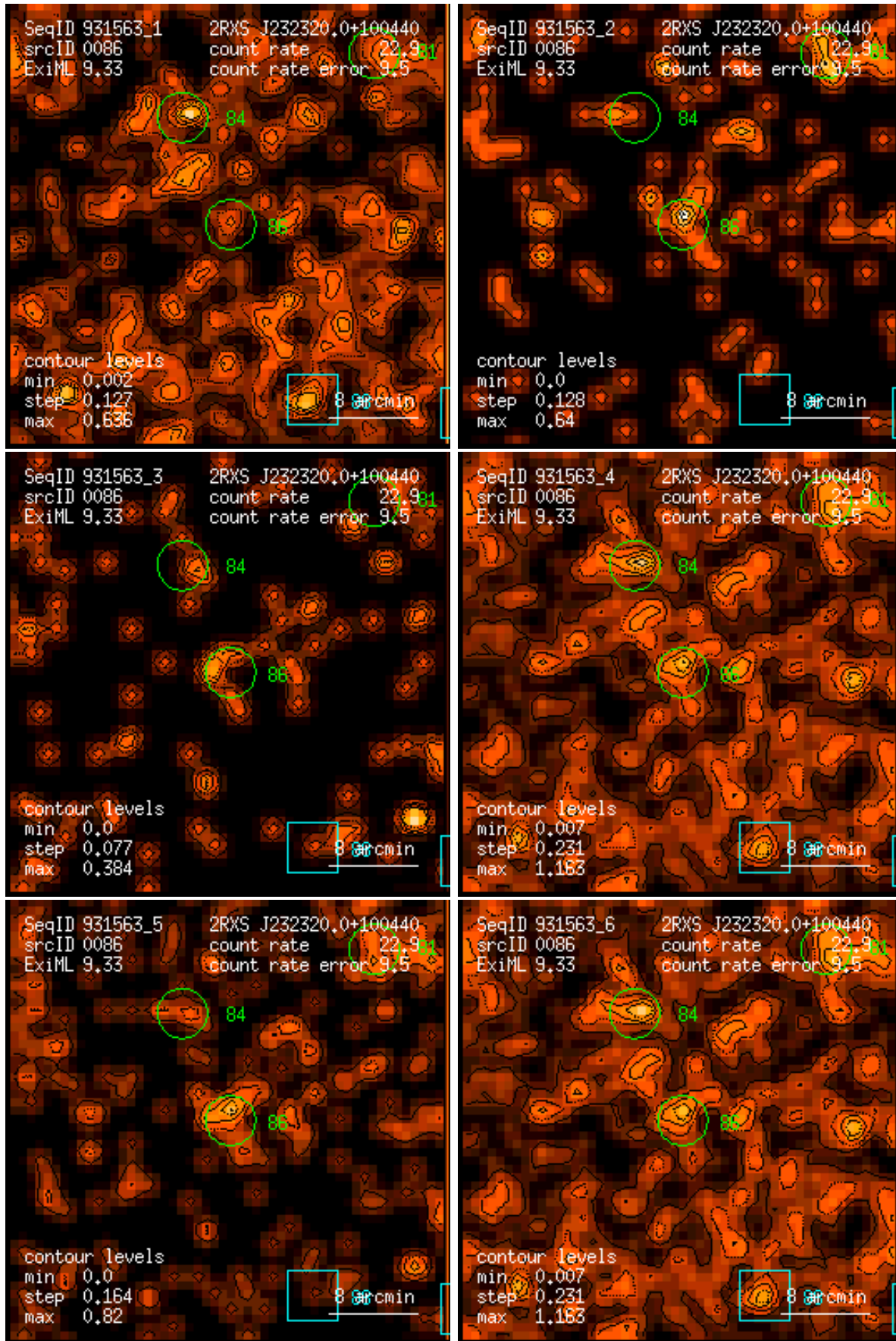
Figure 86: RASS 931563: detection 0086: band rate images, Gaussian filter: (1) PSPC channels 11 – 41, (2) 52 – 90, (3) 91 – 201, (4) 11 – 235, (5) 52 – 201, (6) 11 – 201. Broad band rates in counts/ks. Band rate contour levels in counts/ks/arcmin 2 .
