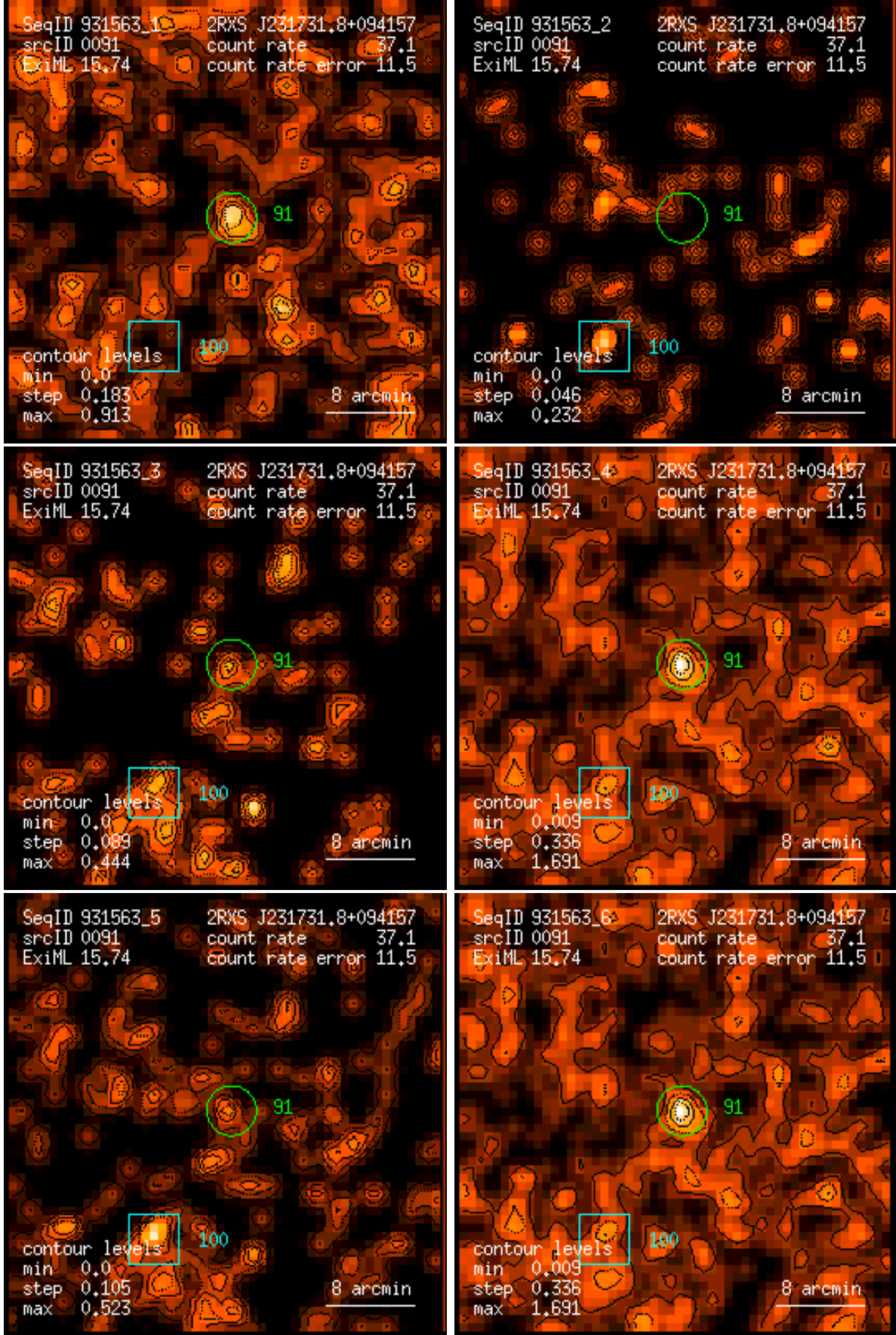
Figure 91: RASS 931563: detection 0091: band rate images, Gaussian filter: (1) PSPC channels 11 – 41, (2) 52 – 90, (3) 91 – 201, (4) 11 – 235, (5) 52 – 201, (6) 11 – 201. Broad band rates in counts/ks. Band rate contour levels in counts/ks/arcmin 2 .
