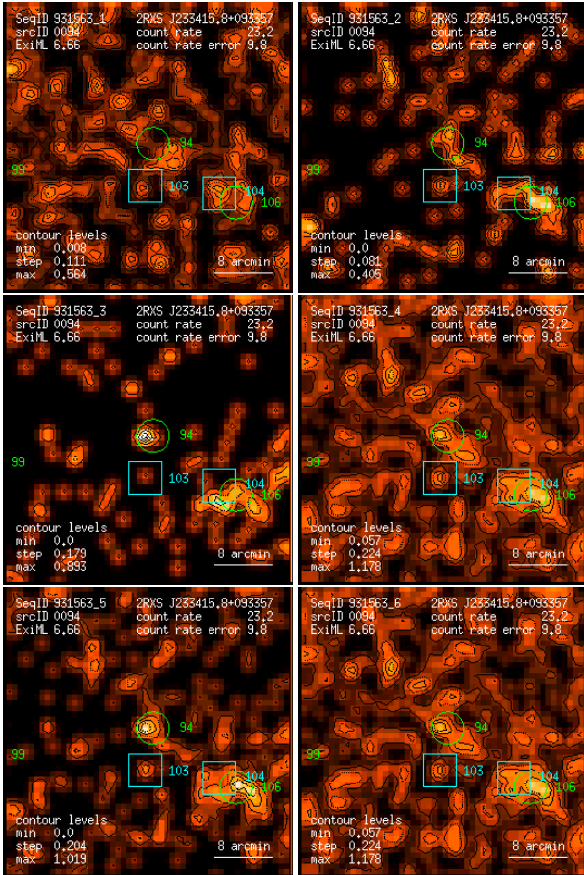
Figure 94: RASS 931563: detection 0094: band rate images, Gaussian filter: (1) PSPC channels 11 – 41, (2) 52 – 90, (3) 91 – 201, (4) 11 – 235, (5) 52 – 201, (6) 11 – 201. Broad band rates in counts/ks. Band rate contour levels in counts/ks/arcmin 2 .
