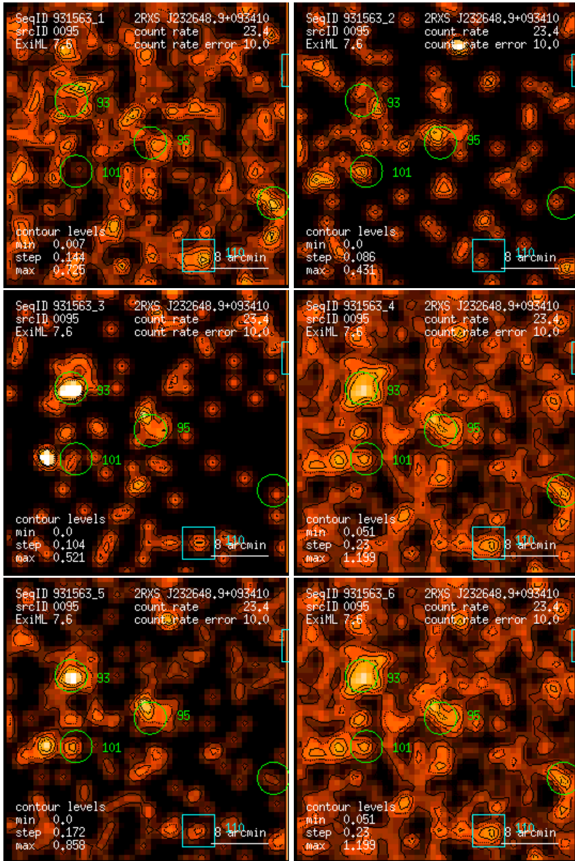
Figure 95: RASS 931563: detection 0095: band rate images, Gaussian filter: (1) PSPC channels 11 – 41, (2) 52 – 90, (3) 91 – 201, (4) 11 – 235, (5) 52 – 201, (6) 11 – 201. Broad band rates in counts/ks. Band rate contour levels in counts/ks/arcmin 2 .
