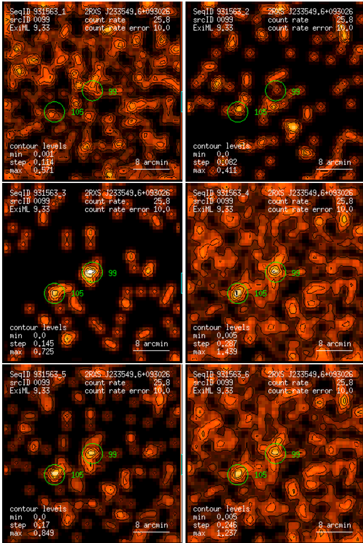
Figure 99: RASS 931563: detection 0099: band rate images, Gaussian filter: (1) PSPC channels 11 – 41, (2) 52 – 90, (3) 91 – 201, (4) 11 – 235, (5) 52 – 201, (6) 11 – 201. Broad band rates in counts/ks. Band rate contour levels in counts/ks/arcmin 2 .
