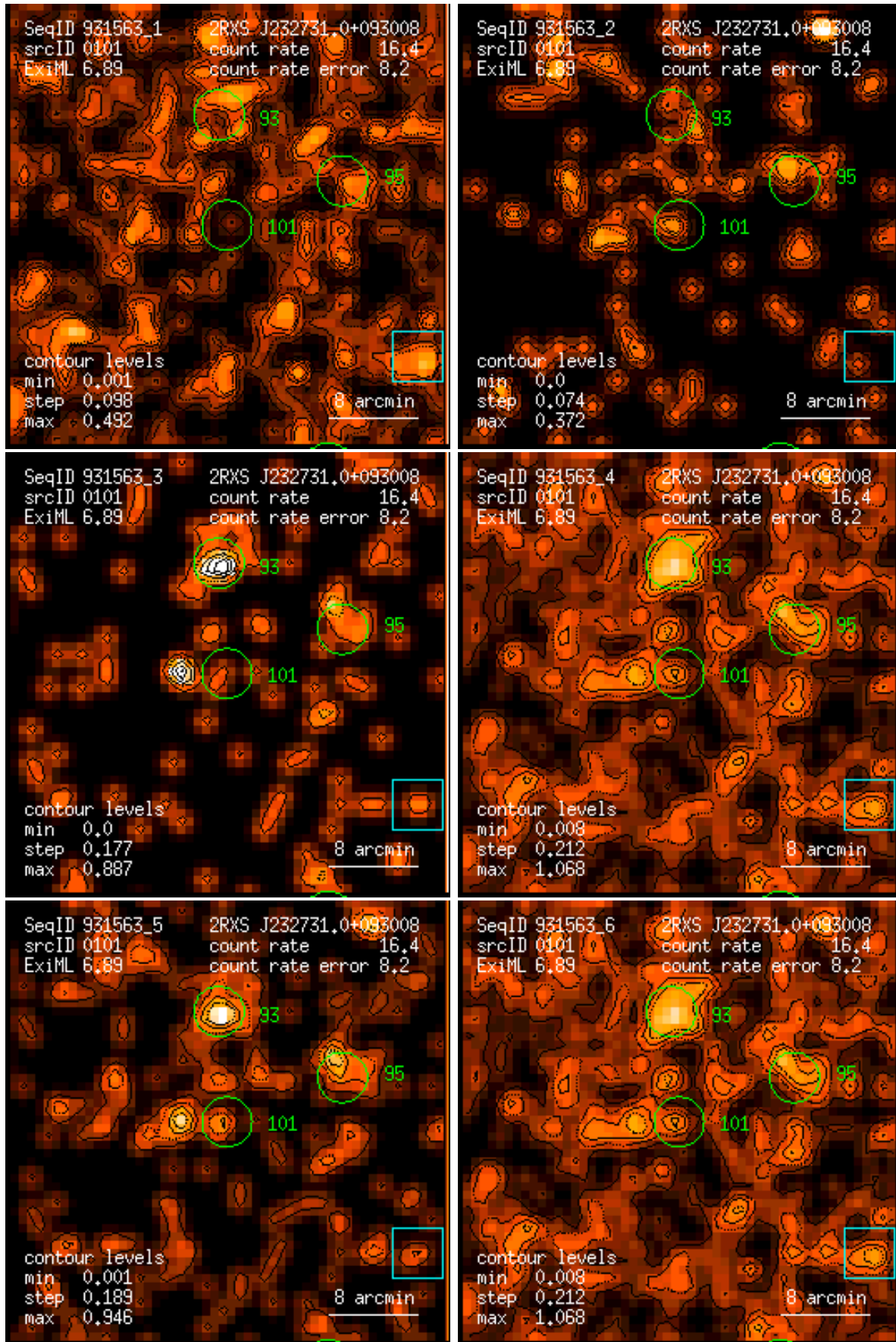
Figure 101: RASS 931563: detection 0101: band rate images, Gaussian filter: (1) PSPC channels 11 – 41, (2) 52 – 90, (3) 91 – 201, (4) 11 – 235, (5) 52 – 201, (6) 11 – 201. Broad band rates in counts/ks. Band rate contour levels in counts/ks/arcmin 2 .
