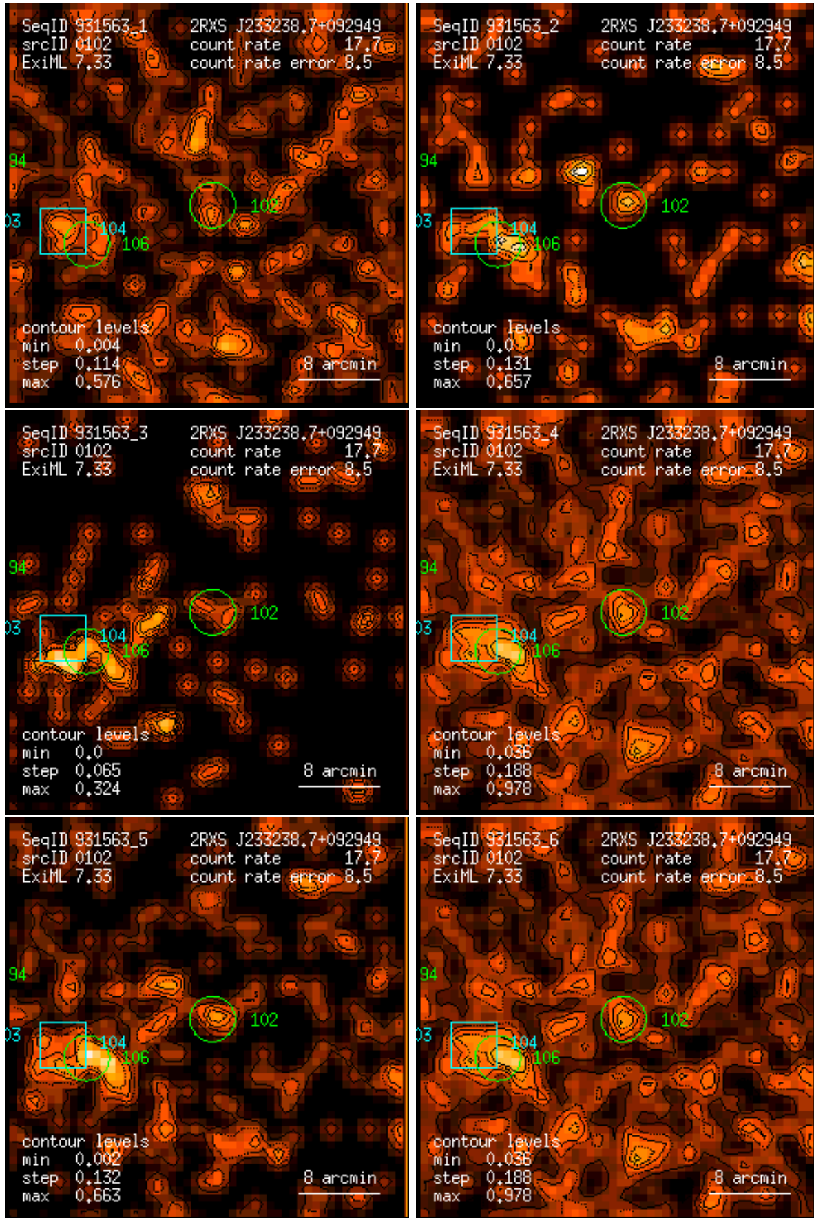
Figure 102: RASS 931563: detection 0102: band rate images, Gaussian filter: (1) PSPC channels 11 – 41, (2) 52 – 90, (3) 91 – 201, (4) 11 – 235, (5) 52 – 201, (6) 11 – 201. Broad band rates in counts/ks. Band rate contour levels in counts/ks/arcmin 2 .
