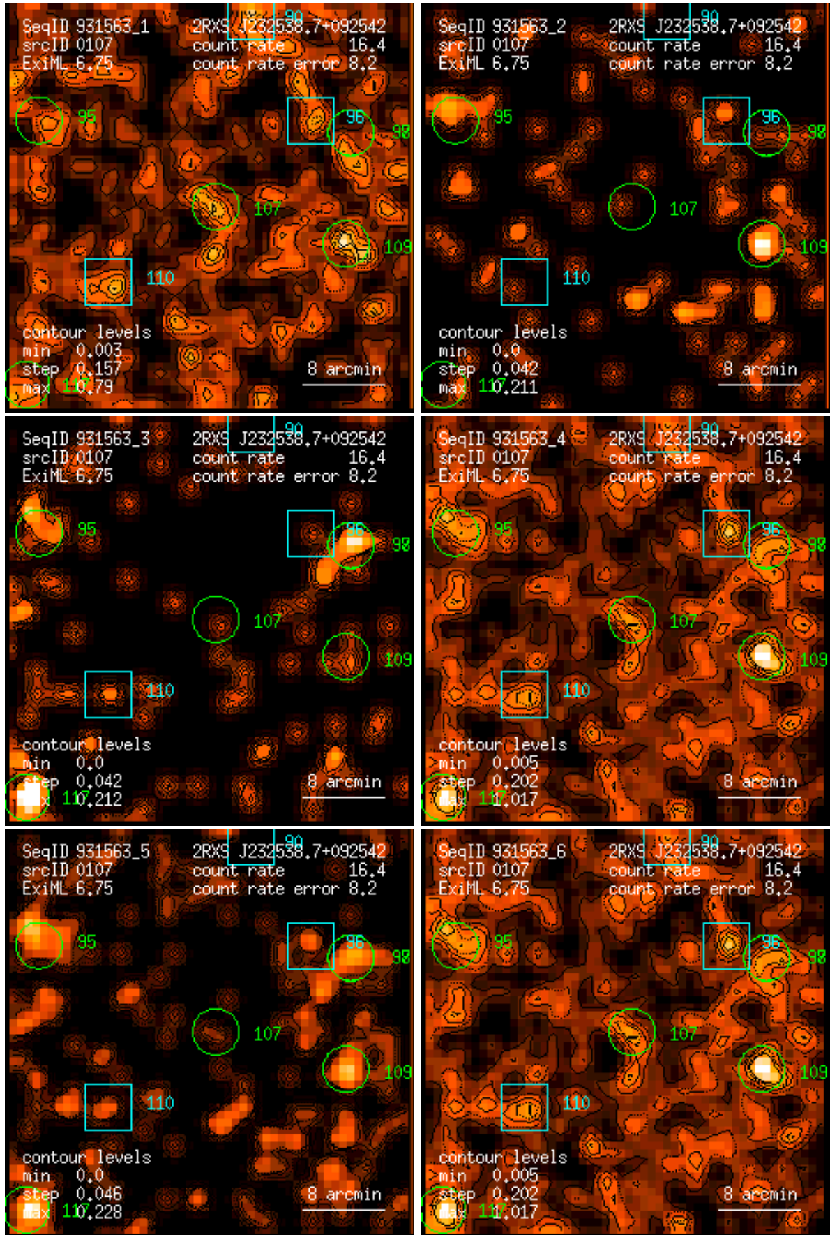
Figure 107: RASS 931563: detection 0107: band rate images, Gaussian filter: (1) PSPC channels 11 – 41, (2) 52 – 90, (3) 91 – 201, (4) 11 – 235, (5) 52 – 201, (6) 11 – 201. Broad band rates in counts/ks. Band rate contour levels in counts/ks/arcmin 2 .
