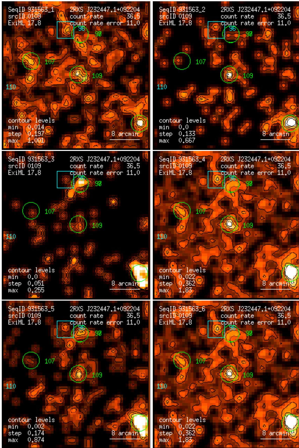
Figure 109: RASS 931563: detection 0109: band rate images, Gaussian filter: (1) PSPC channels 11 – 41, (2) 52 – 90, (3) 91 – 201, (4) 11 – 235, (5) 52 – 201, (6) 11 – 201. Broad band rates in counts/ks. Band rate contour levels in counts/ks/arcmin 2 .
