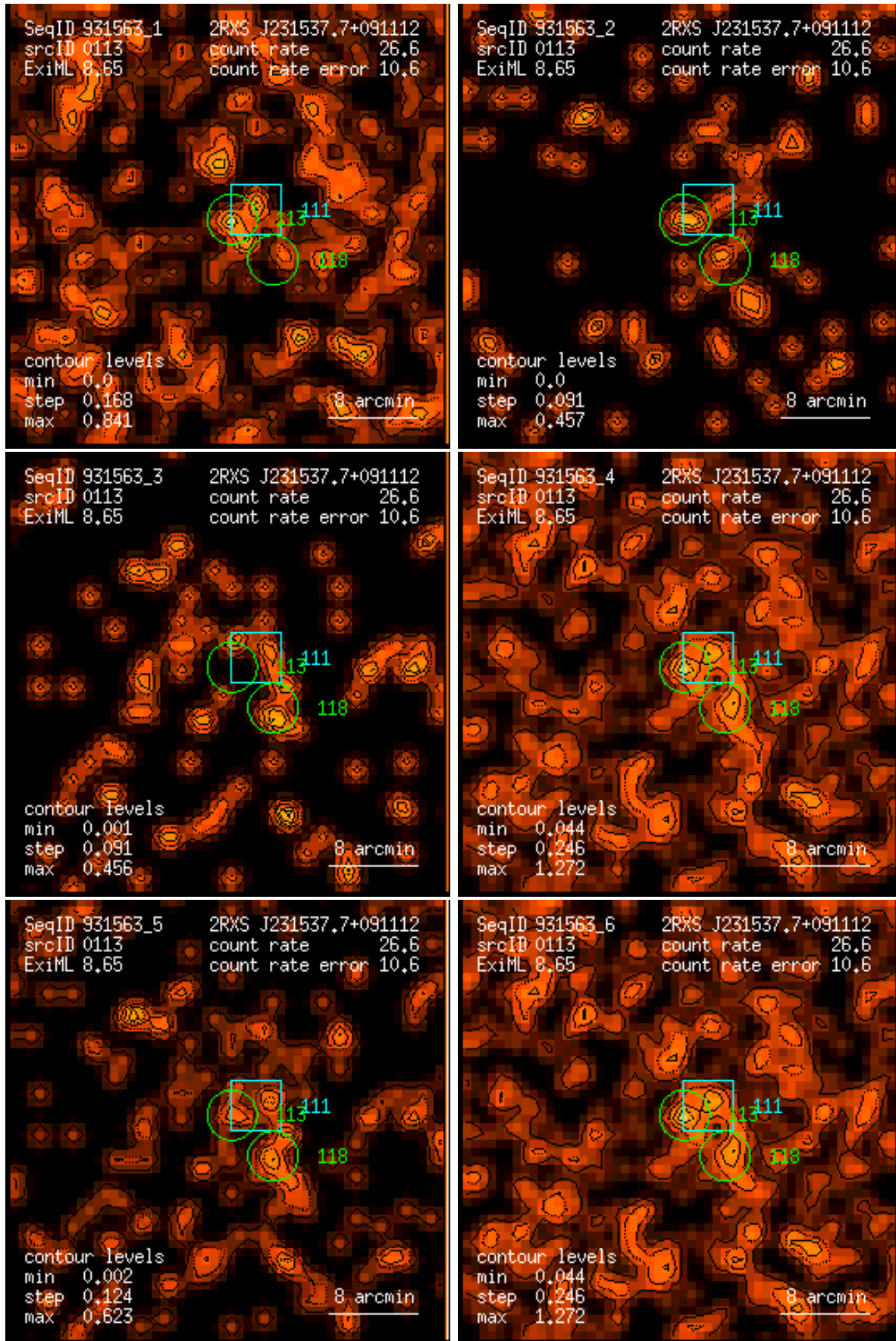
Figure 113: RASS 931563: detection 0113: band rate images, Gaussian filter: (1) PSPC channels 11 – 41, (2) 52 – 90, (3) 91 – 201, (4) 11 – 235, (5) 52 – 201, (6) 11 – 201. Broad band rates in counts/ks. Band rate contour levels in counts/ks/arcmin 2 .
