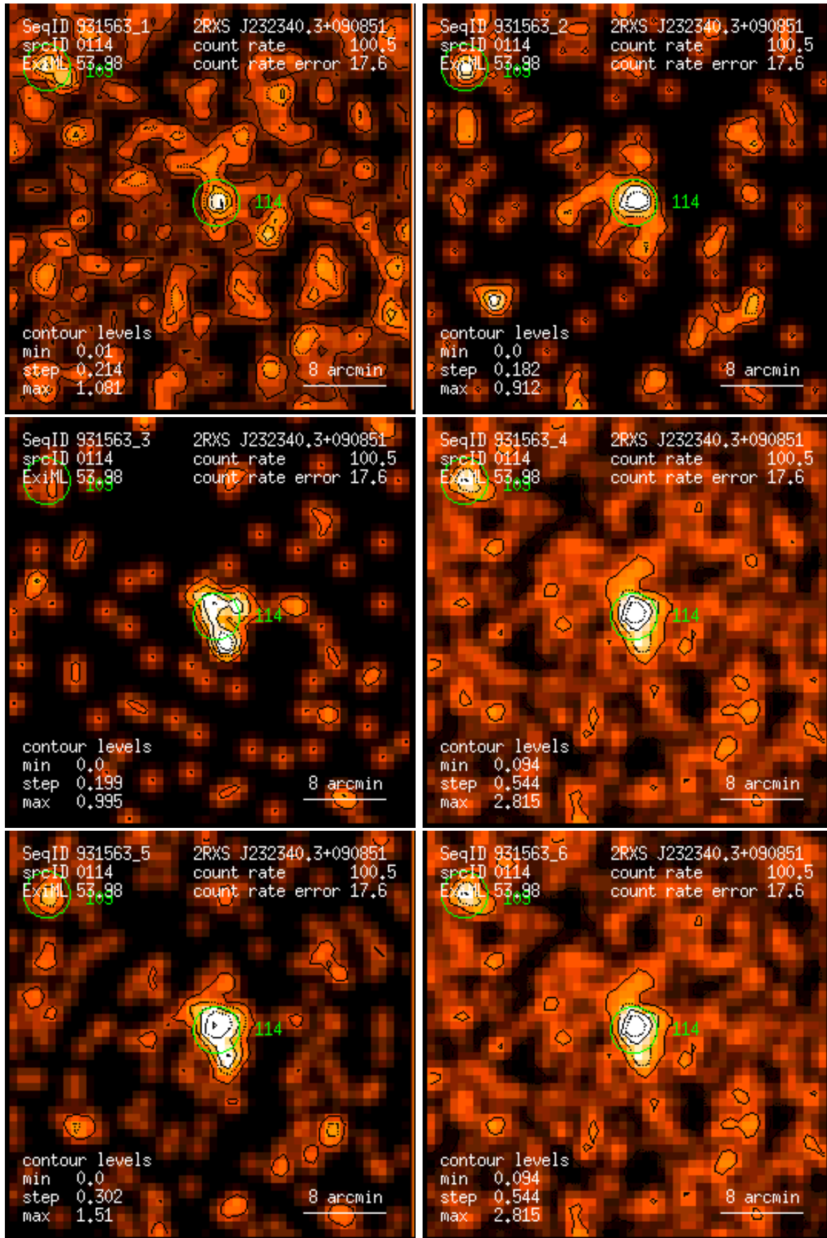
Figure 114: RASS 931563: detection 0114: band rate images, Gaussian filter: (1) PSPC channels 11 – 41, (2) 52 – 90, (3) 91 – 201, (4) 11 – 235, (5) 52 – 201, (6) 11 – 201. Broad band rates in counts/ks. Band rate contour levels in counts/ks/arcmin 2 .
