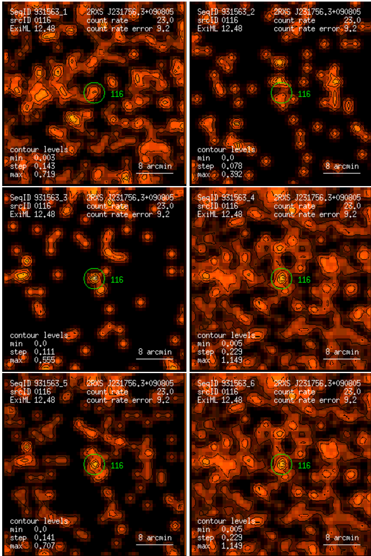
Figure 116: RASS 931563: detection 0116: band rate images, Gaussian filter: (1) PSPC channels 11 – 41, (2) 52 – 90, (3) 91 – 201, (4) 11 – 235, (5) 52 – 201, (6) 11 – 201. Broad band rates in counts/ks. Band rate contour levels in counts/ks/arcmin 2 .
