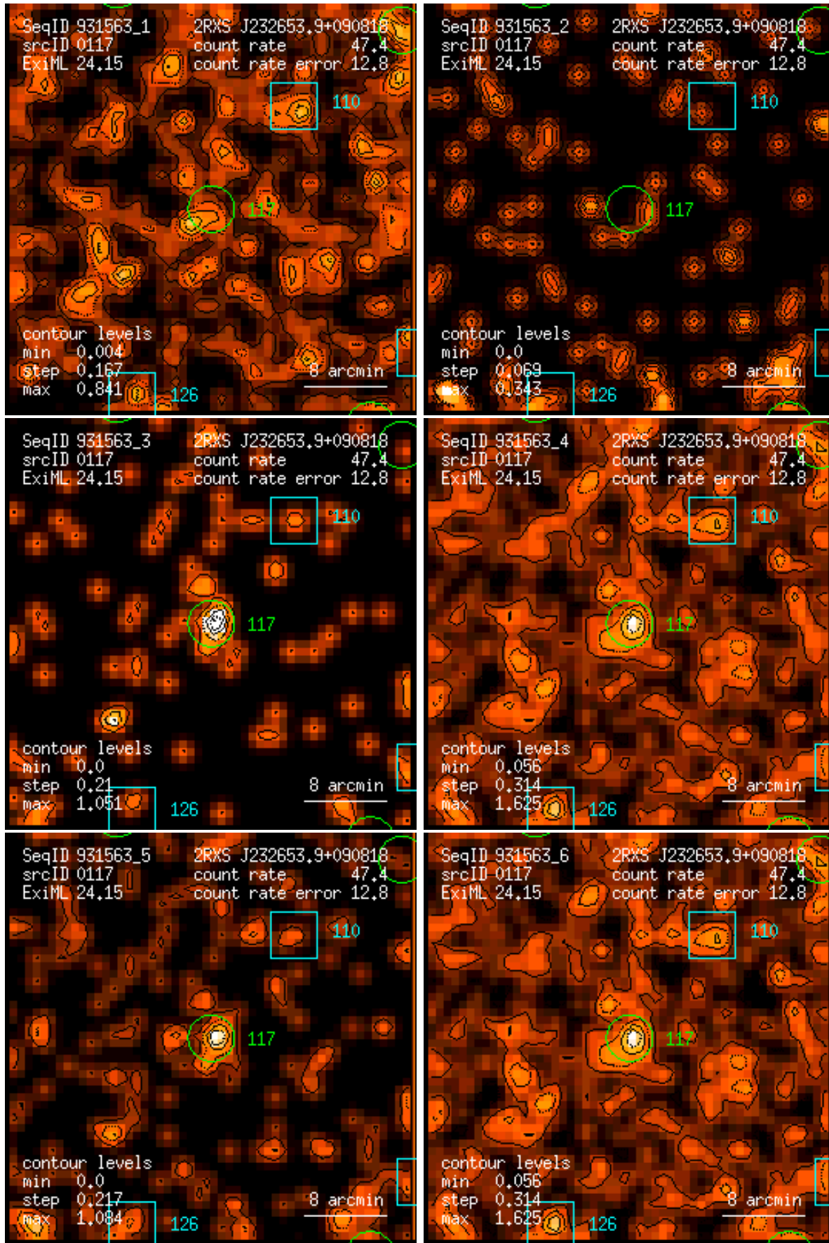
Figure 117: RASS 931563: detection 0117: band rate images, Gaussian filter: (1) PSPC channels 11 – 41, (2) 52 – 90, (3) 91 – 201, (4) 11 – 235, (5) 52 – 201, (6) 11 – 201. Broad band rates in counts/ks. Band rate contour levels in counts/ks/arcmin 2 .
