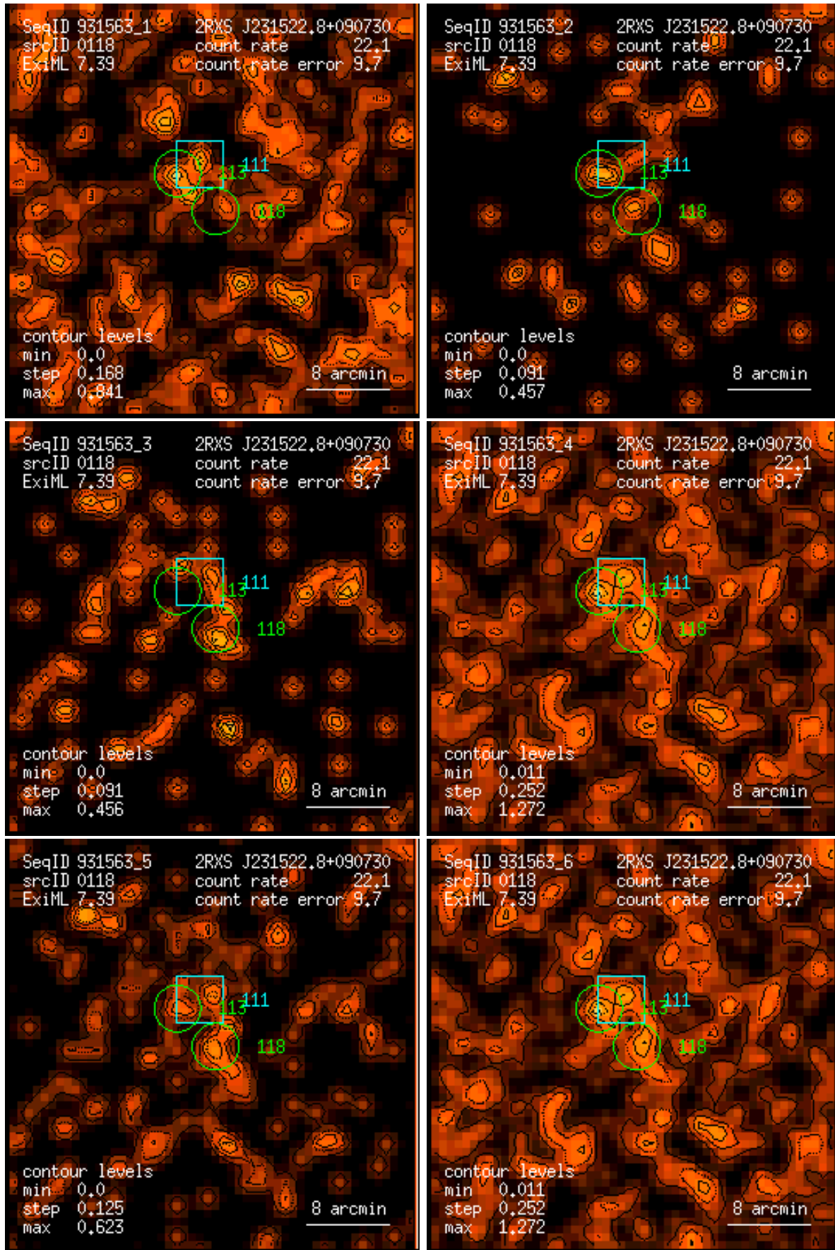
Figure 118: RASS 931563: detection 0118: band rate images, Gaussian filter: (1) PSPC channels 11 – 41, (2) 52 – 90, (3) 91 – 201, (4) 11 – 235, (5) 52 – 201, (6) 11 – 201. Broad band rates in counts/ks. Band rate contour levels in counts/ks/arcmin 2 .
