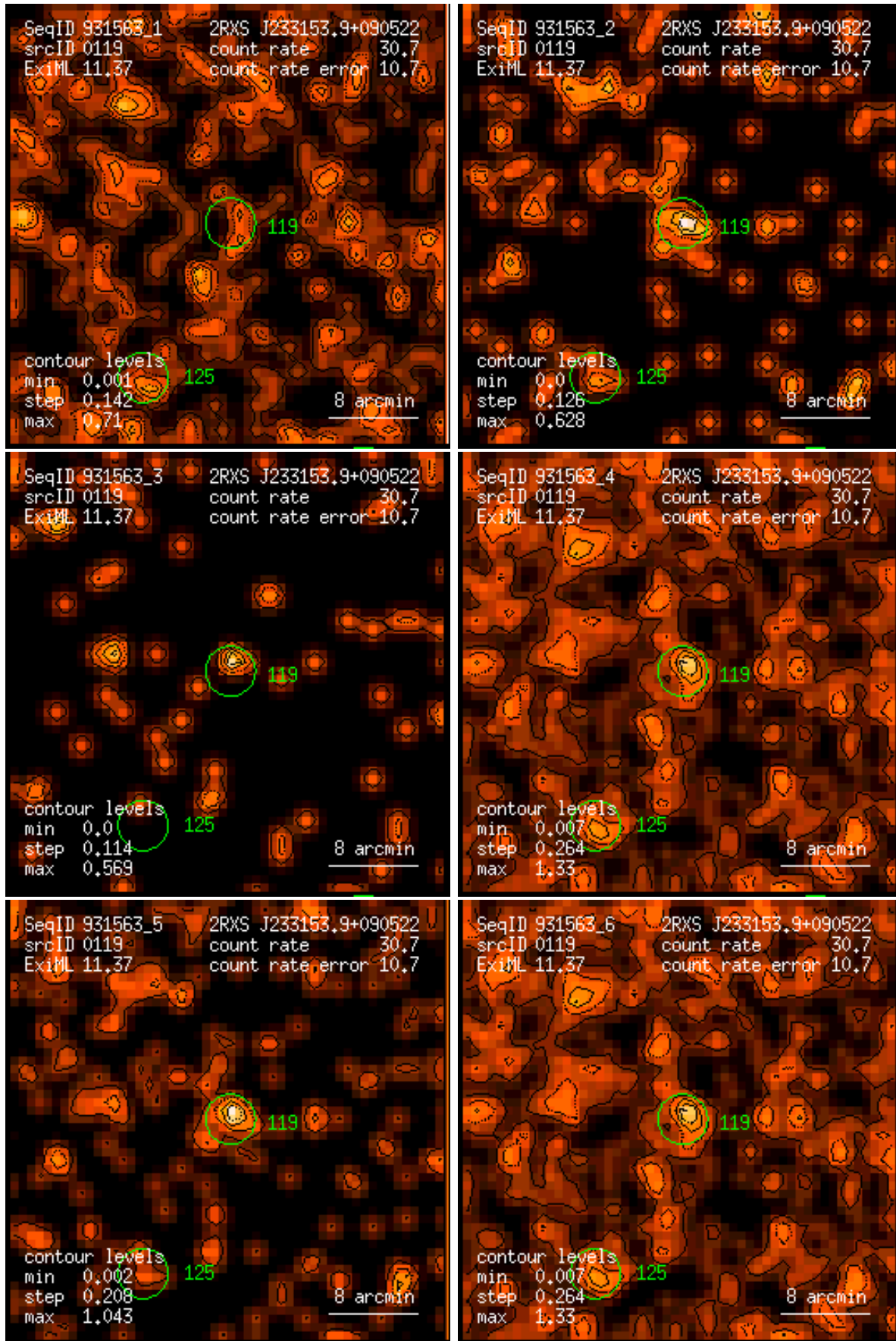
Figure 119: RASS 931563: detection 0119: band rate images, Gaussian filter: (1) PSPC channels 11 – 41, (2) 52 – 90, (3) 91 – 201, (4) 11 – 235, (5) 52 – 201, (6) 11 – 201. Broad band rates in counts/ks. Band rate contour levels in counts/ks/arcmin 2 .
