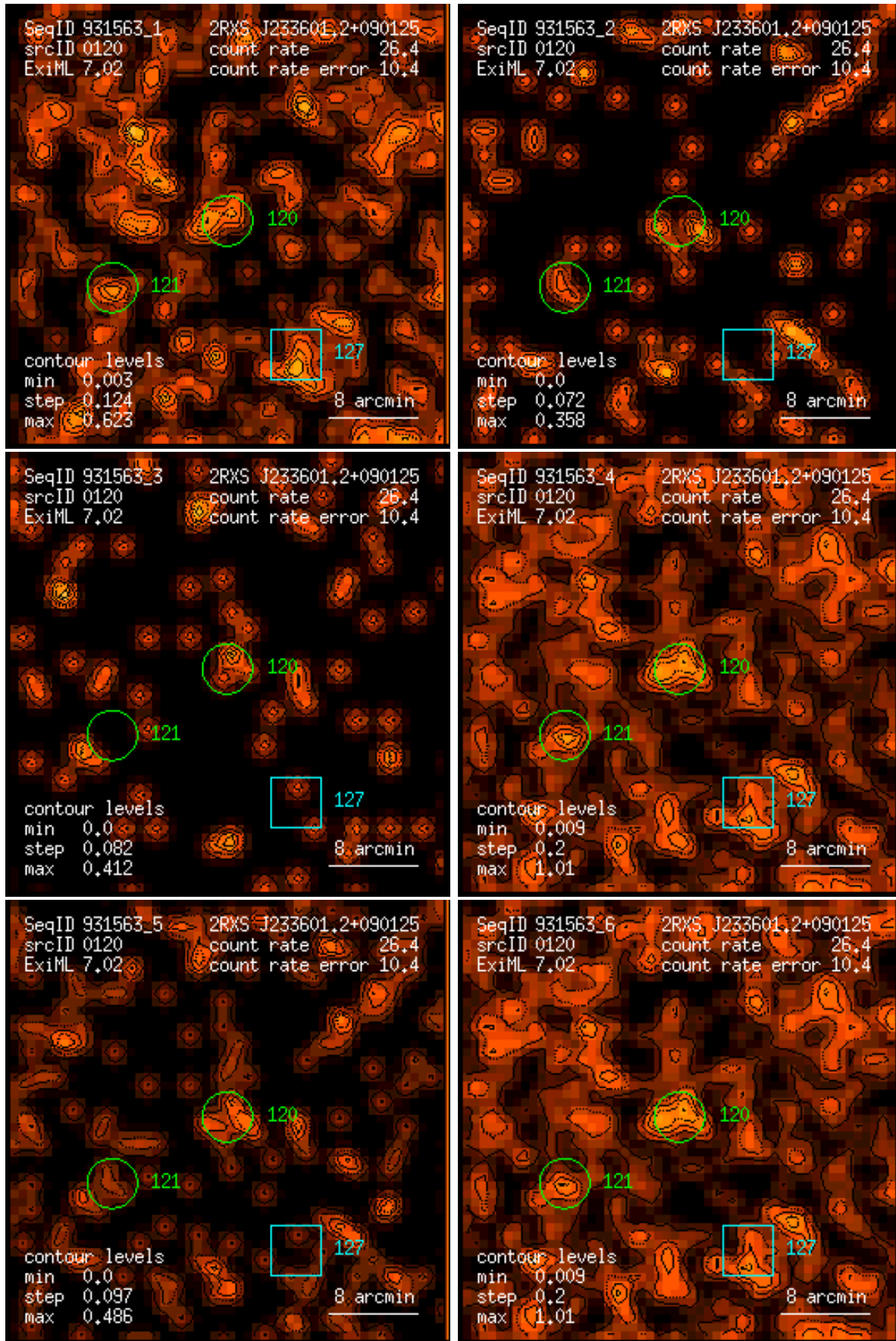
Figure 120: RASS 931563: detection 0120: band rate images, Gaussian filter: (1) PSPC channels 11 – 41, (2) 52 – 90, (3) 91 – 201, (4) 11 – 235, (5) 52 – 201, (6) 11 – 201. Broad band rates in counts/ks. Band rate contour levels in counts/ks/arcmin 2 .
