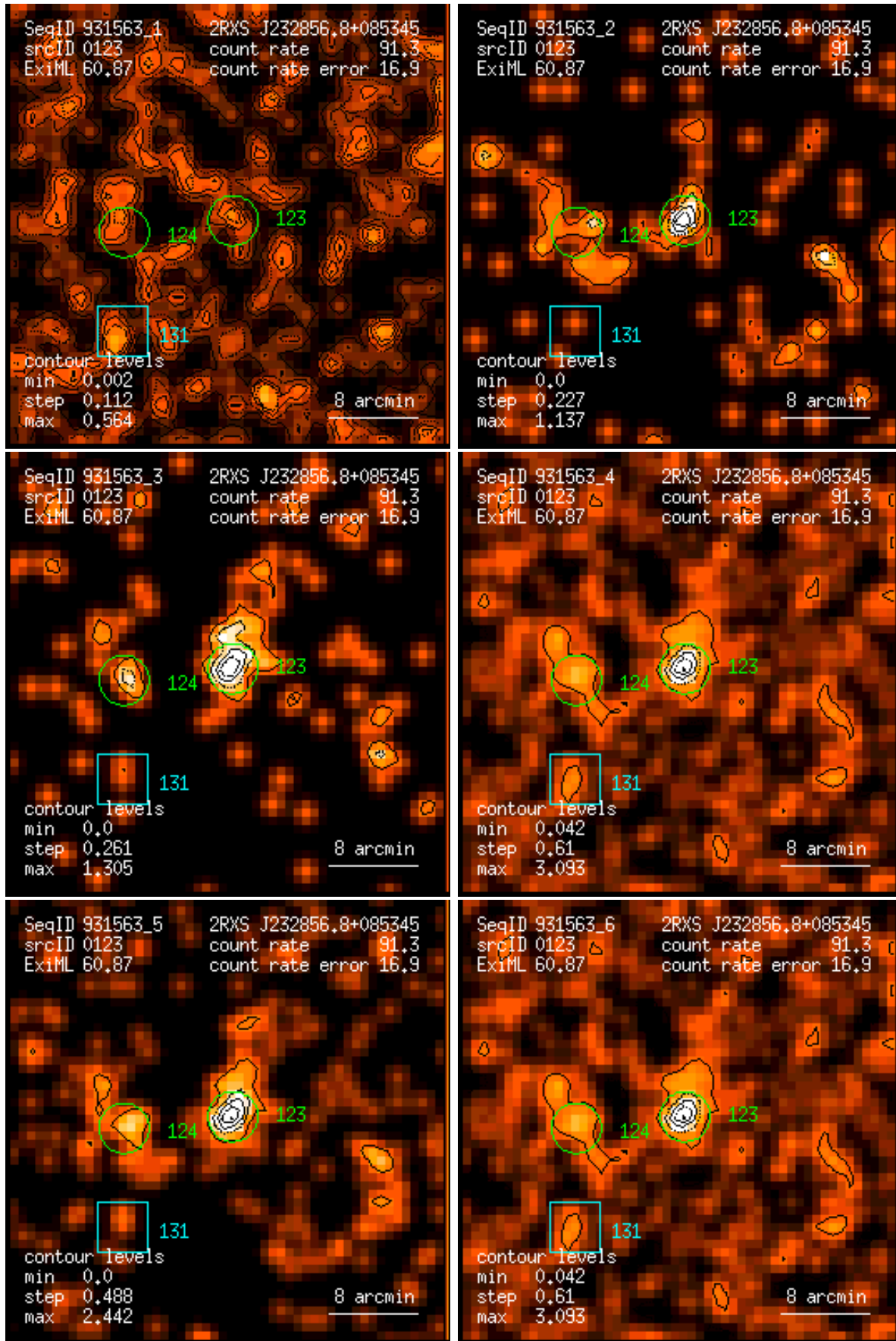
Figure 123: RASS 931563: detection 0123: band rate images, Gaussian filter: (1) PSPC channels 11 – 41, (2) 52 – 90, (3) 91 – 201, (4) 11 – 235, (5) 52 – 201, (6) 11 – 201. Broad band rates in counts/ks. Band rate contour levels in counts/ks/arcmin 2 .
