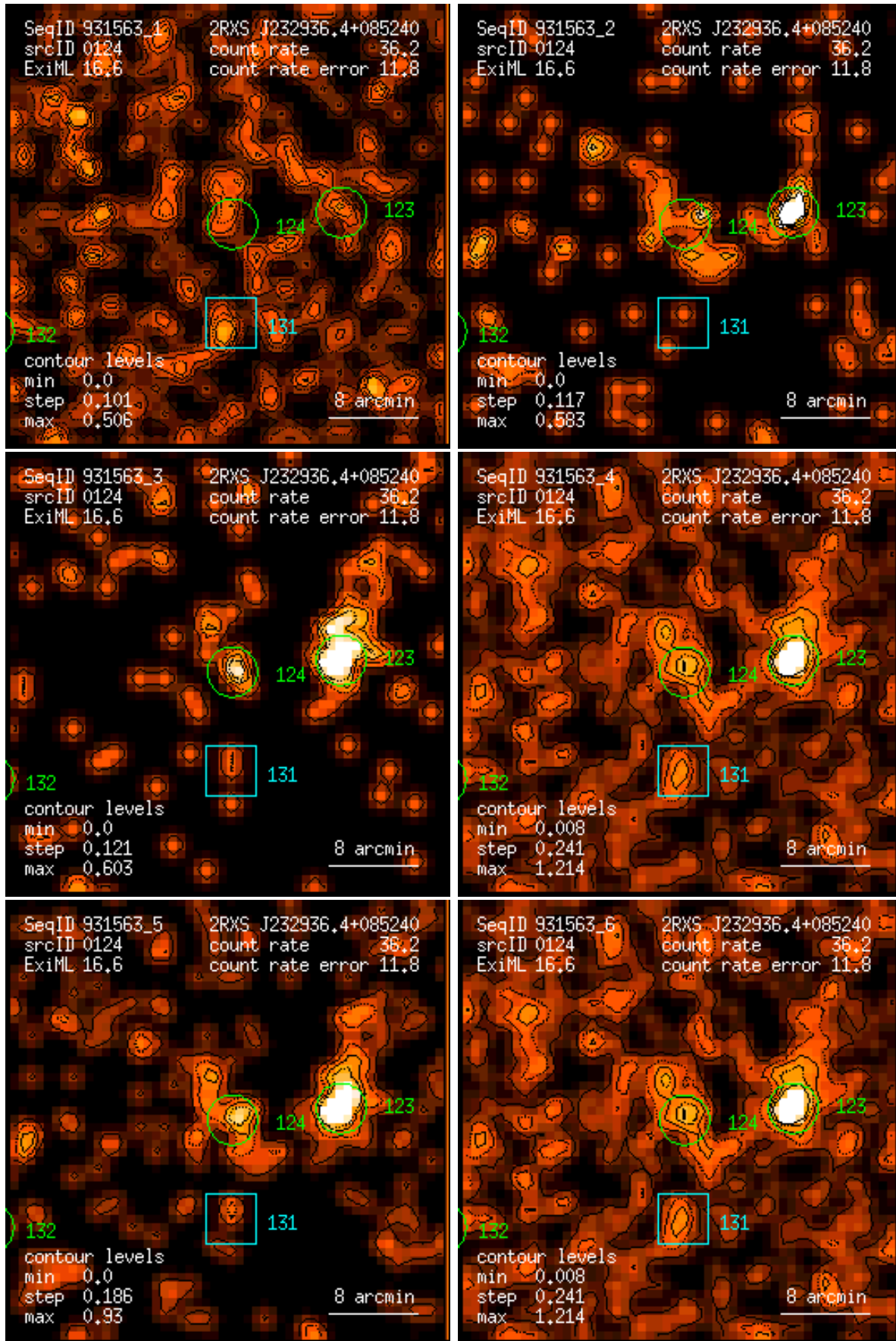
Figure 124: RASS 931563: detection 0124: band rate images, Gaussian filter: (1) PSPC channels 11 – 41, (2) 52 – 90, (3) 91 – 201, (4) 11 – 235, (5) 52 – 201, (6) 11 – 201. Broad band rates in counts/ks. Band rate contour levels in counts/ks/arcmin 2 .
