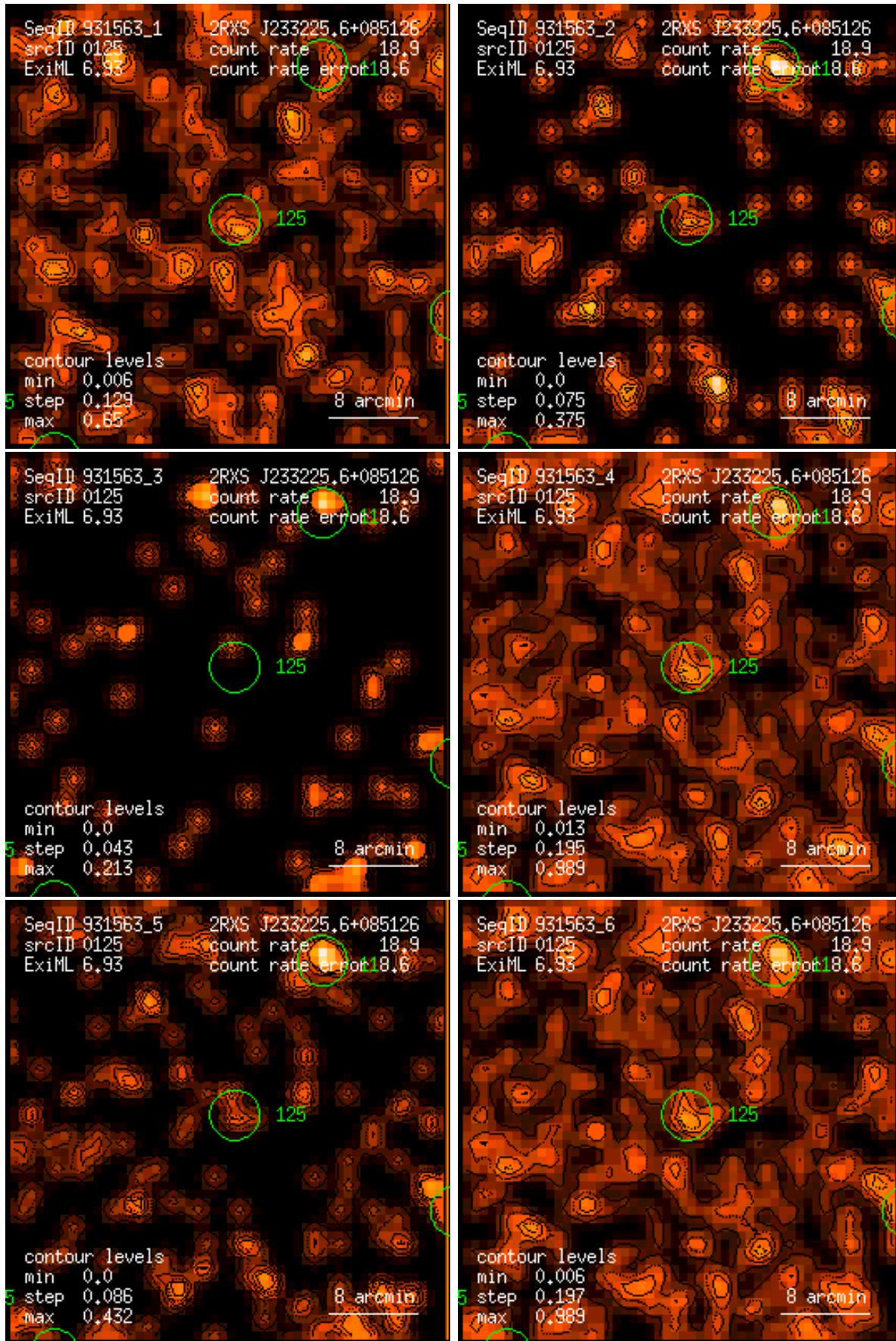
Figure 125: RASS 931563: detection 0125: band rate images, Gaussian filter: (1) PSPC channels 11 – 41, (2) 52 – 90, (3) 91 – 201, (4) 11 – 235, (5) 52 – 201, (6) 11 – 201. Broad band rates in counts/ks. Band rate contour levels in counts/ks/arcmin 2 .
