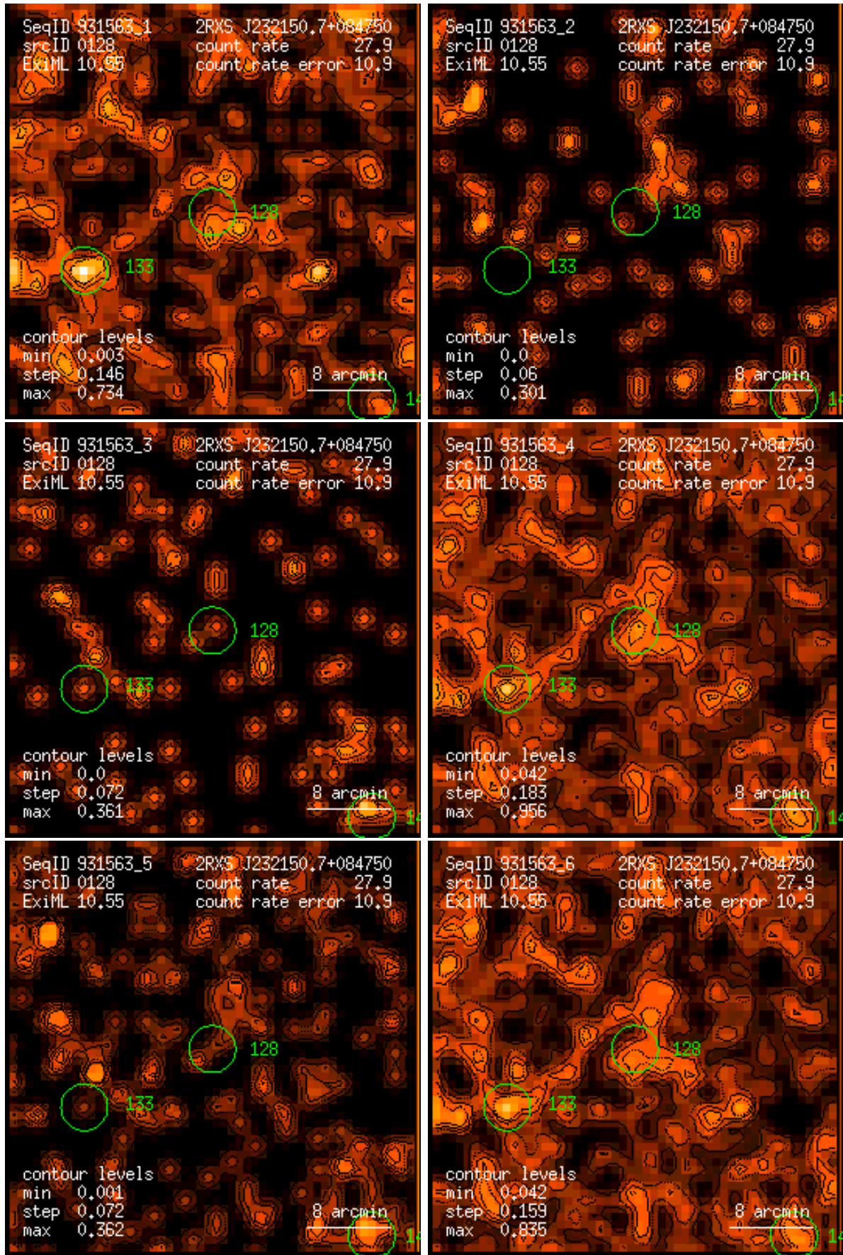
Figure 128: RASS 931563: detection 0128: band rate images, Gaussian filter: (1) PSPC channels 11 – 41, (2) 52 – 90, (3) 91 – 201, (4) 11 – 235, (5) 52 – 201, (6) 11 – 201. Broad band rates in counts/ks. Band rate contour levels in counts/ks/arcmin 2 .
