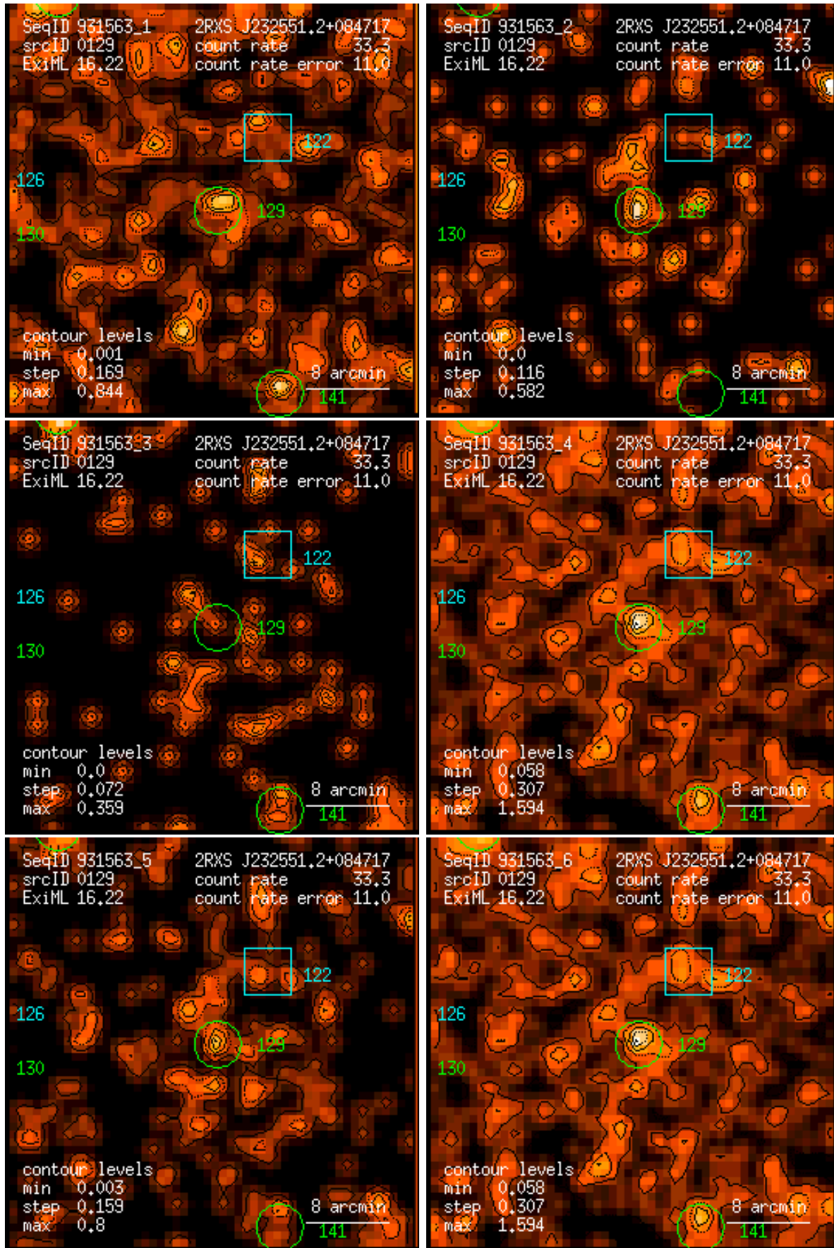
Figure 129: RASS 931563: detection 0129: band rate images, Gaussian filter: (1) PSPC channels 11 – 41, (2) 52 – 90, (3) 91 – 201, (4) 11 – 235, (5) 52 – 201, (6) 11 – 201. Broad band rates in counts/ks. Band rate contour levels in counts/ks/arcmin 2 .
