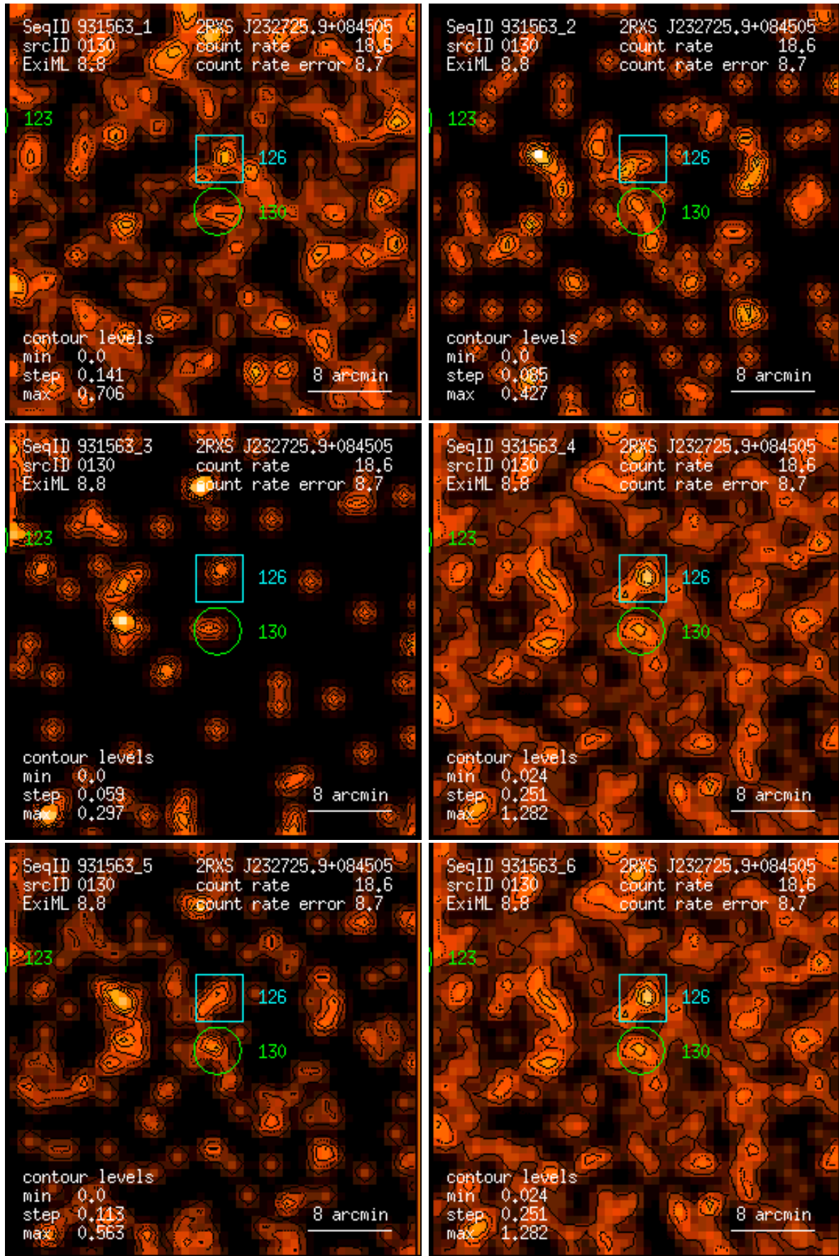
Figure 130: RASS 931563: detection 0130: band rate images, Gaussian filter: (1) PSPC channels 11 – 41, (2) 52 – 90, (3) 91 – 201, (4) 11 – 235, (5) 52 – 201, (6) 11 – 201. Broad band rates in counts/ks. Band rate contour levels in counts/ks/arcmin 2 .
