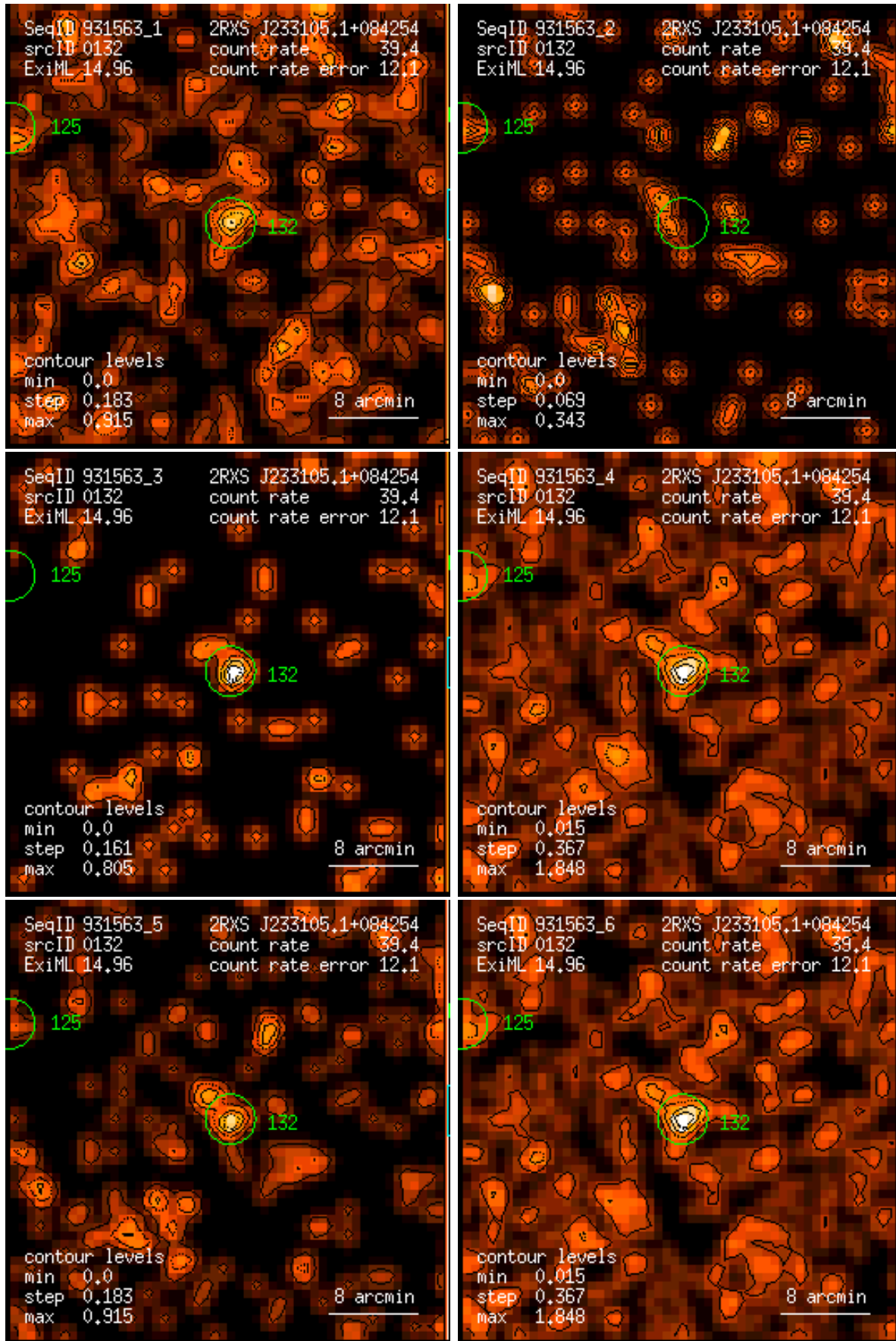
Figure 132: RASS 931563: detection 0132: band rate images, Gaussian filter: (1) PSPC channels 11 – 41, (2) 52 – 90, (3) 91 – 201, (4) 11 – 235, (5) 52 – 201, (6) 11 – 201. Broad band rates in counts/ks. Band rate contour levels in counts/ks/arcmin 2 .
