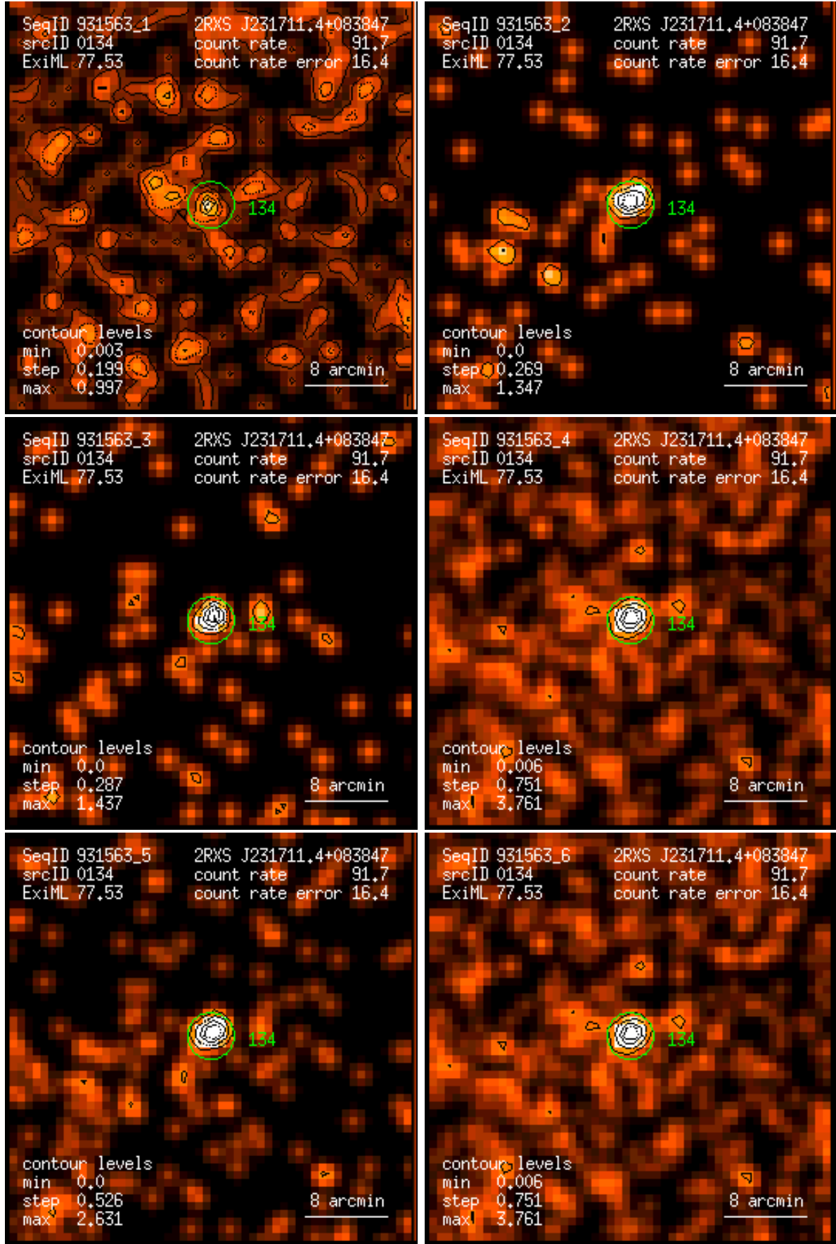
Figure 134: RASS 931563: detection 0134: band rate images, Gaussian filter: (1) PSPC channels 11 – 41, (2) 52 – 90, (3) 91 – 201, (4) 11 – 235, (5) 52 – 201, (6) 11 – 201. Broad band rates in counts/ks. Band rate contour levels in counts/ks/arcmin 2 .
