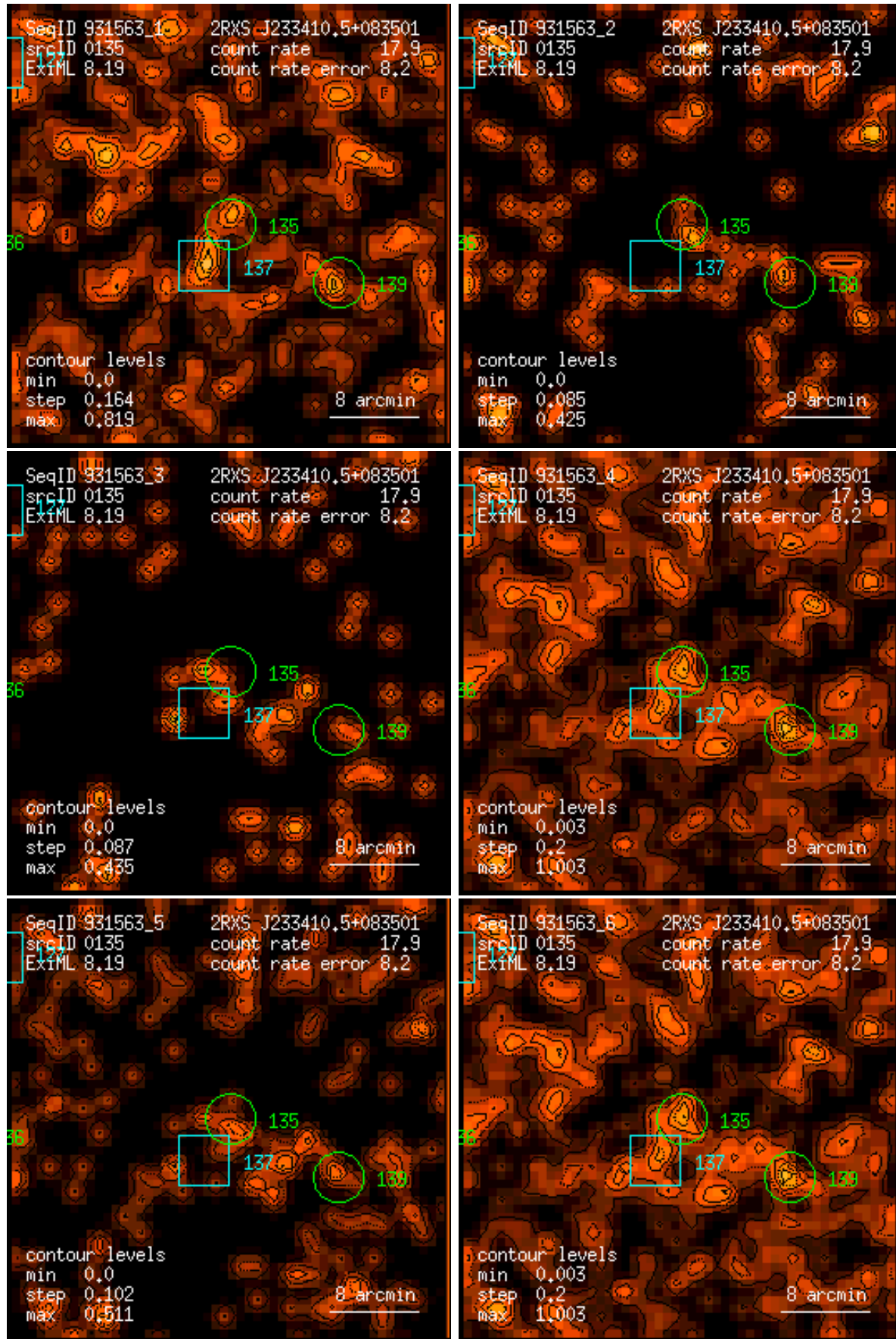
Figure 135: RASS 931563: detection 0135: band rate images, Gaussian filter: (1) PSPC channels 11 – 41, (2) 52 – 90, (3) 91 – 201, (4) 11 – 235, (5) 52 – 201, (6) 11 – 201. Broad band rates in counts/ks. Band rate contour levels in counts/ks/arcmin 2 .
