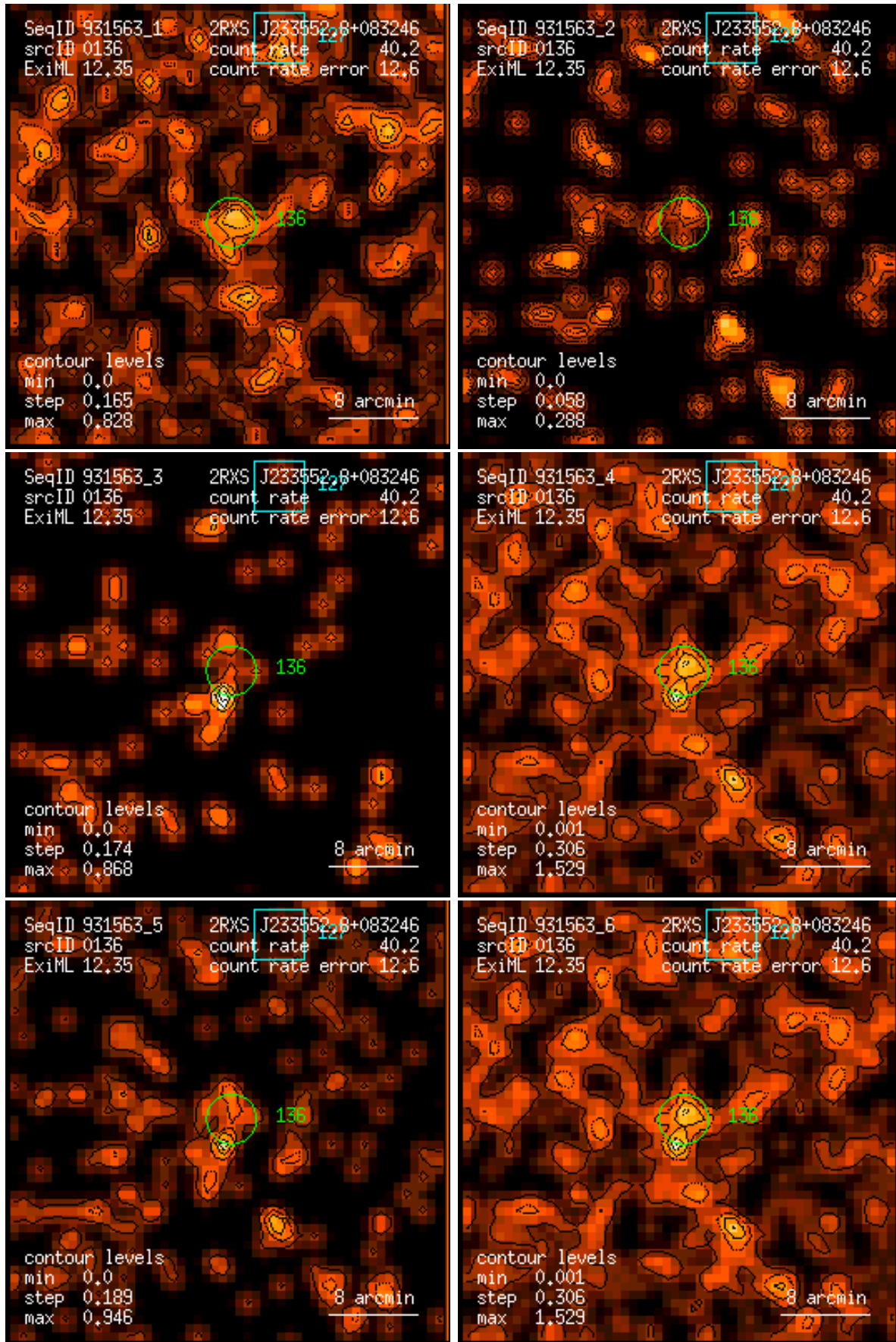
Figure 136: RASS 931563: detection 0136: band rate images, Gaussian filter: (1) PSPC channels 11 – 41, (2) 52 – 90, (3) 91 – 201, (4) 11 – 235, (5) 52 – 201, (6) 11 – 201. Broad band rates in counts/ks. Band rate contour levels in counts/ks/arcmin 2 .
