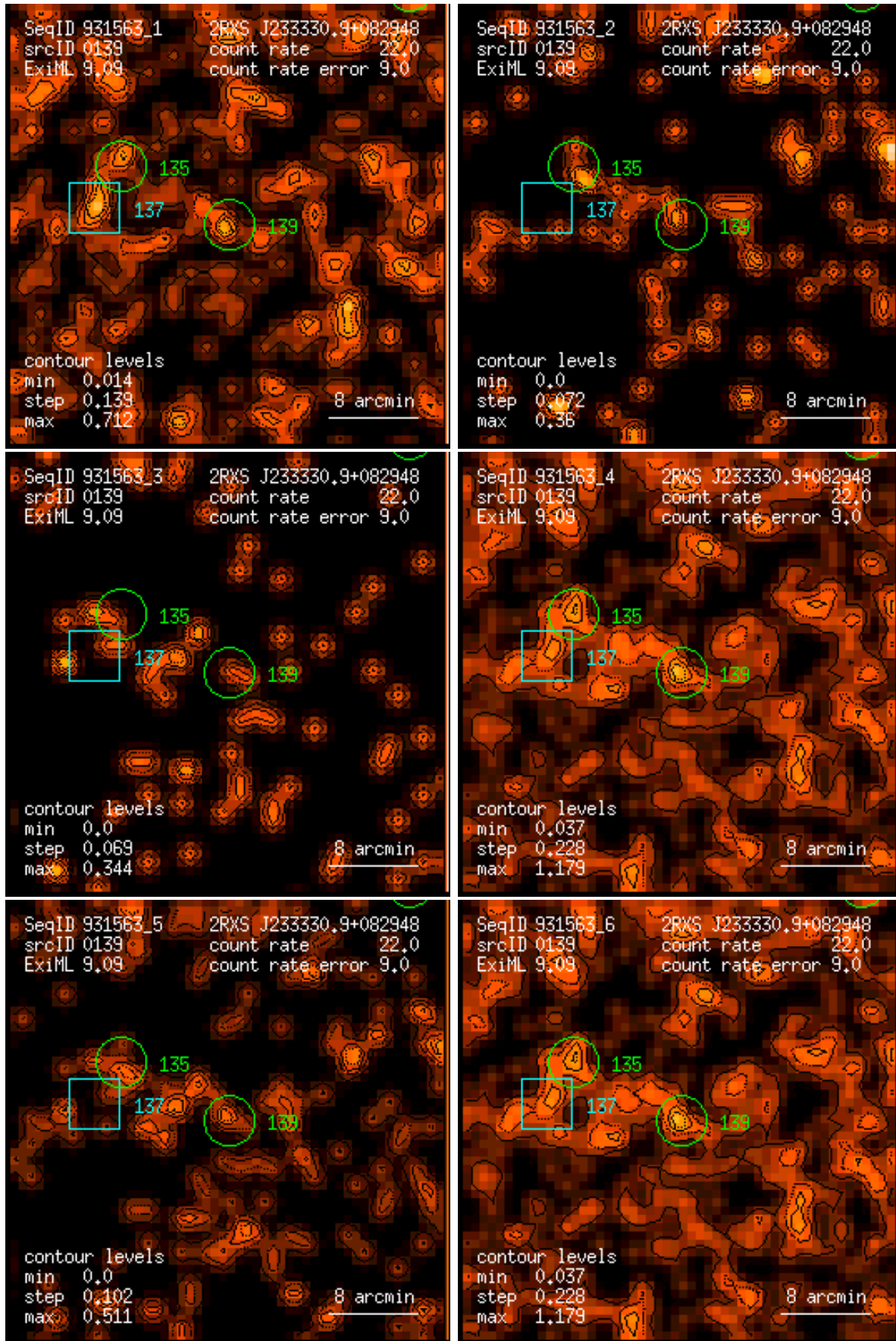
Figure 139: RASS 931563: detection 0139: band rate images, Gaussian filter: (1) PSPC channels 11 – 41, (2) 52 – 90, (3) 91 – 201, (4) 11 – 235, (5) 52 – 201, (6) 11 – 201. Broad band rates in counts/ks. Band rate contour levels in counts/ks/arcmin 2 .
