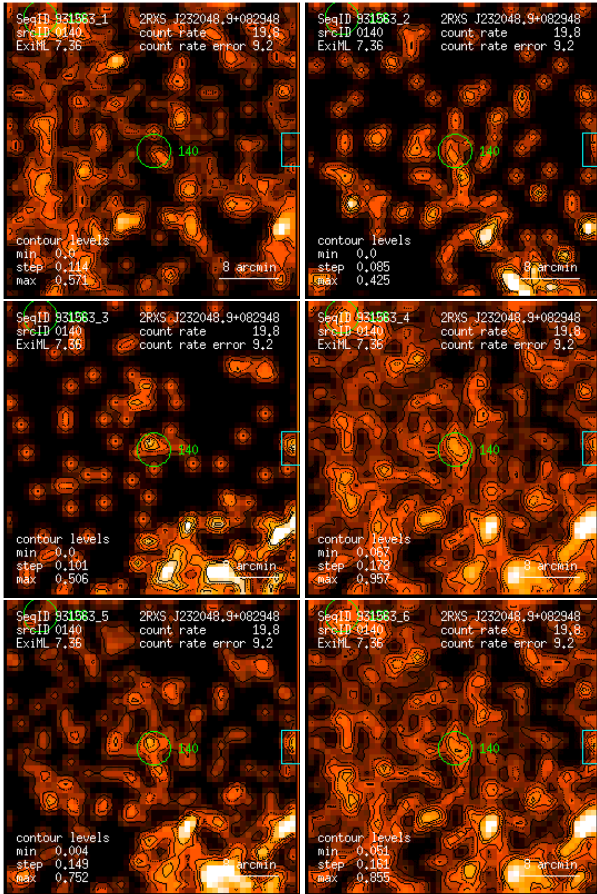
Figure 140: RASS 931563: detection 0140: band rate images, Gaussian filter: (1) PSPC channels 11 – 41, (2) 52 – 90, (3) 91 – 201, (4) 11 – 235, (5) 52 – 201, (6) 11 – 201. Broad band rates in counts/ks. Band rate contour levels in counts/ks/arcmin 2 .
