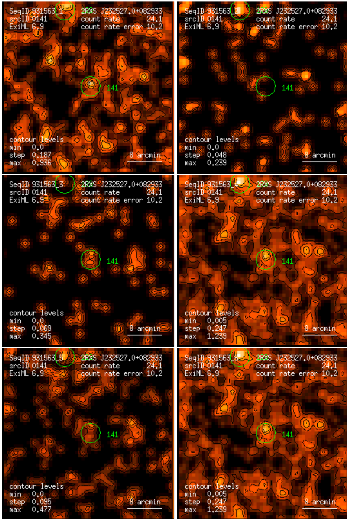
Figure 141: RASS 931563: detection 0141: band rate images, Gaussian filter: (1) PSPC channels 11 – 41, (2) 52 – 90, (3) 91 – 201, (4) 11 – 235, (5) 52 – 201, (6) 11 – 201. Broad band rates in counts/ks. Band rate contour levels in counts/ks/arcmin 2 .
