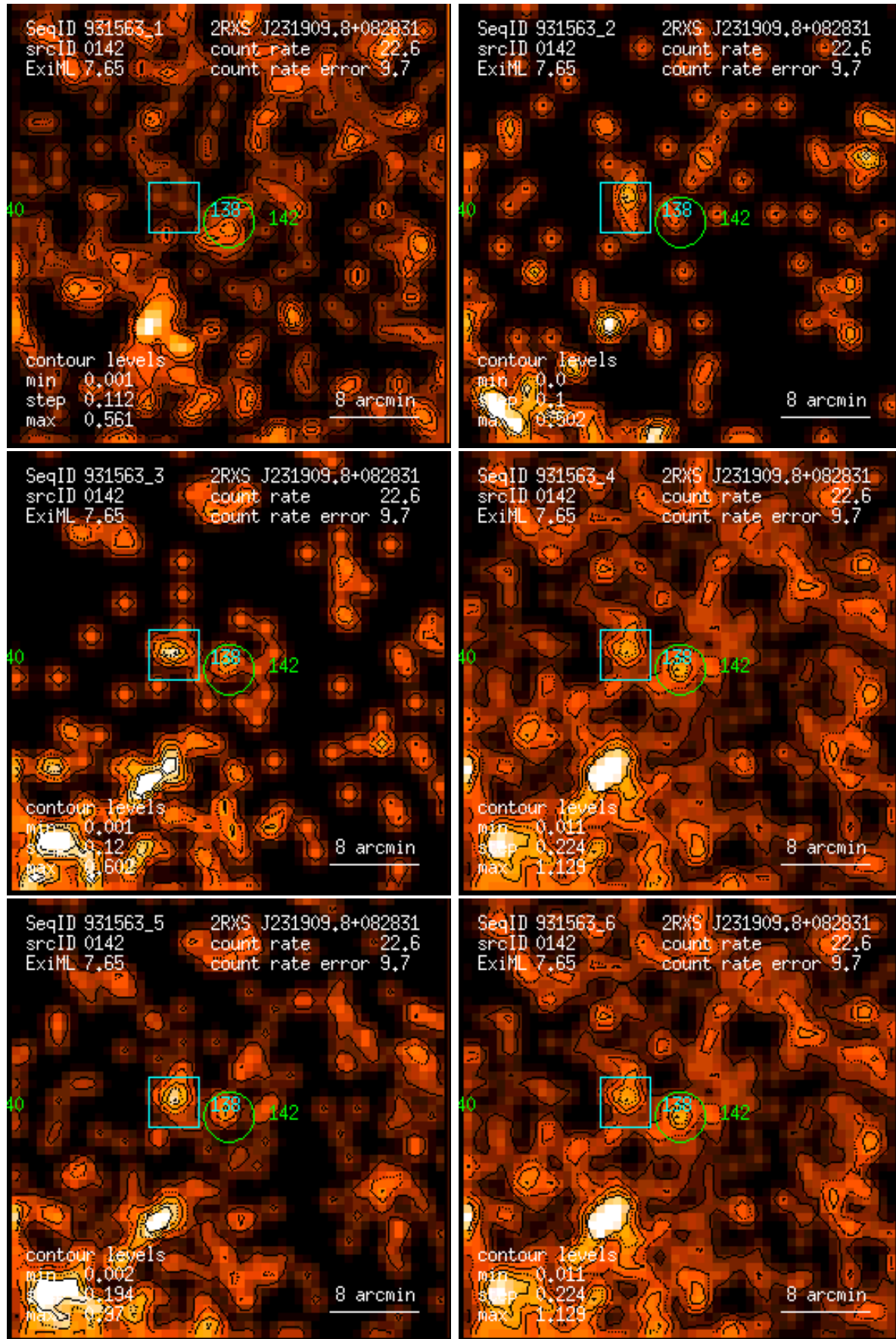
Figure 142: RASS 931563: detection 0142: band rate images, Gaussian filter: (1) PSPC channels 11 – 41, (2) 52 – 90, (3) 91 – 201, (4) 11 – 235, (5) 52 – 201, (6) 11 – 201. Broad band rates in counts/ks. Band rate contour levels in counts/ks/arcmin 2 .
