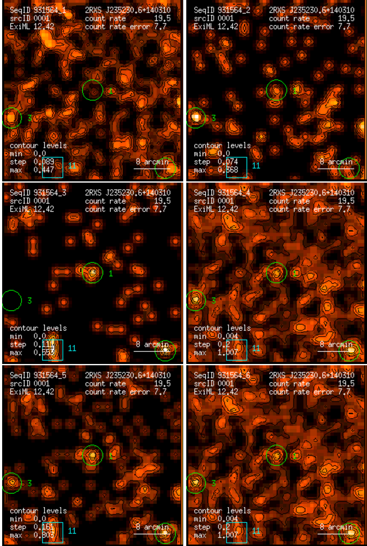
Figure 1: RASS 931564: detection 0001: band rate images, Gaussian filter: (1) PSPC channels 11 – 41, (2) 52 – 90, (3) 91 – 201, (4) 11 – 235, (5) 52 – 201, (6) 11 – 201. Broad band rates in counts/ks. Band rate contour levels in counts/ks/arcmin 2 .
