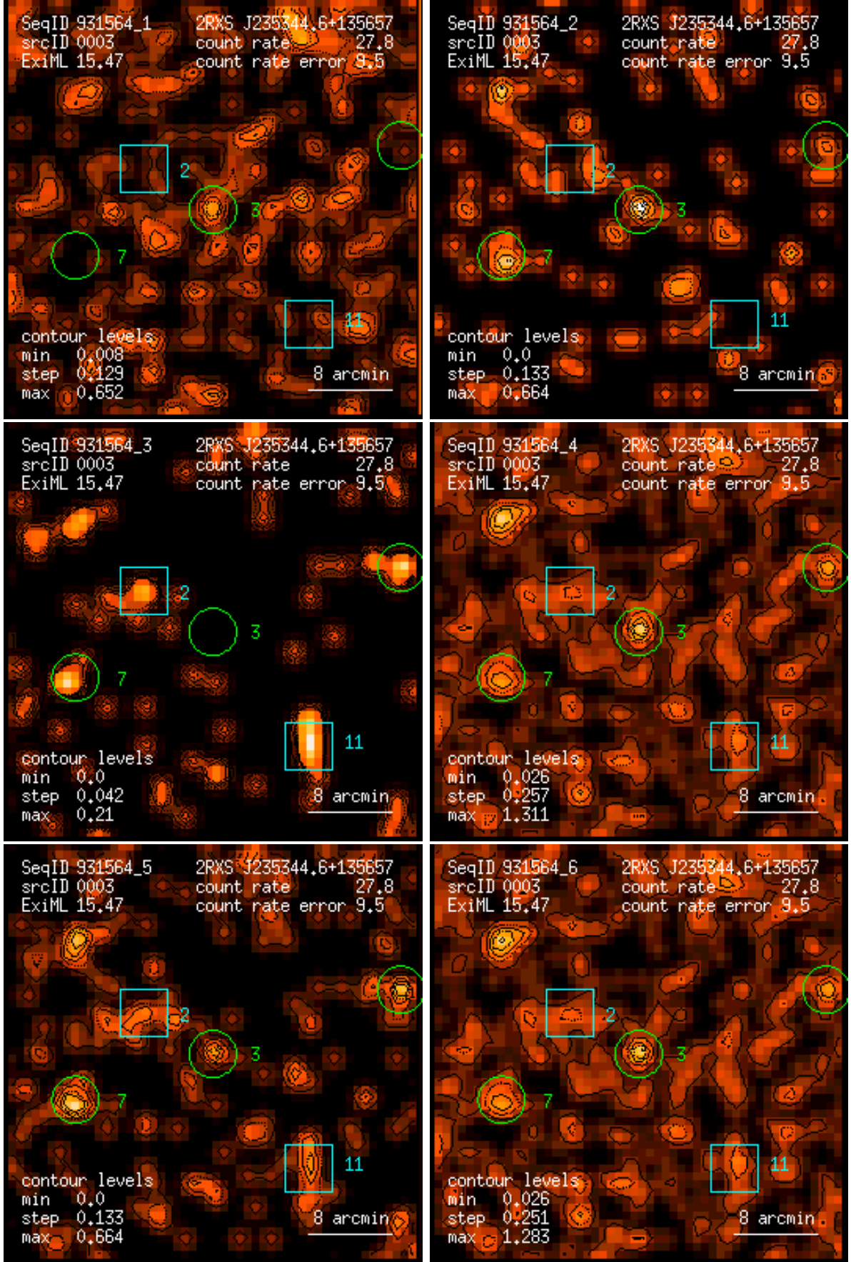
Figure 3: RASS 931564: detection 0003: band rate images, Gaussian filter: (1) PSPC channels 11 – 41, (2) 52 – 90, (3) 91 – 201, (4) 11 – 235, (5) 52 – 201, (6) 11 – 201. Broad band rates in counts/ks. Band rate contour levels in counts/ks/arcmin 2 .
