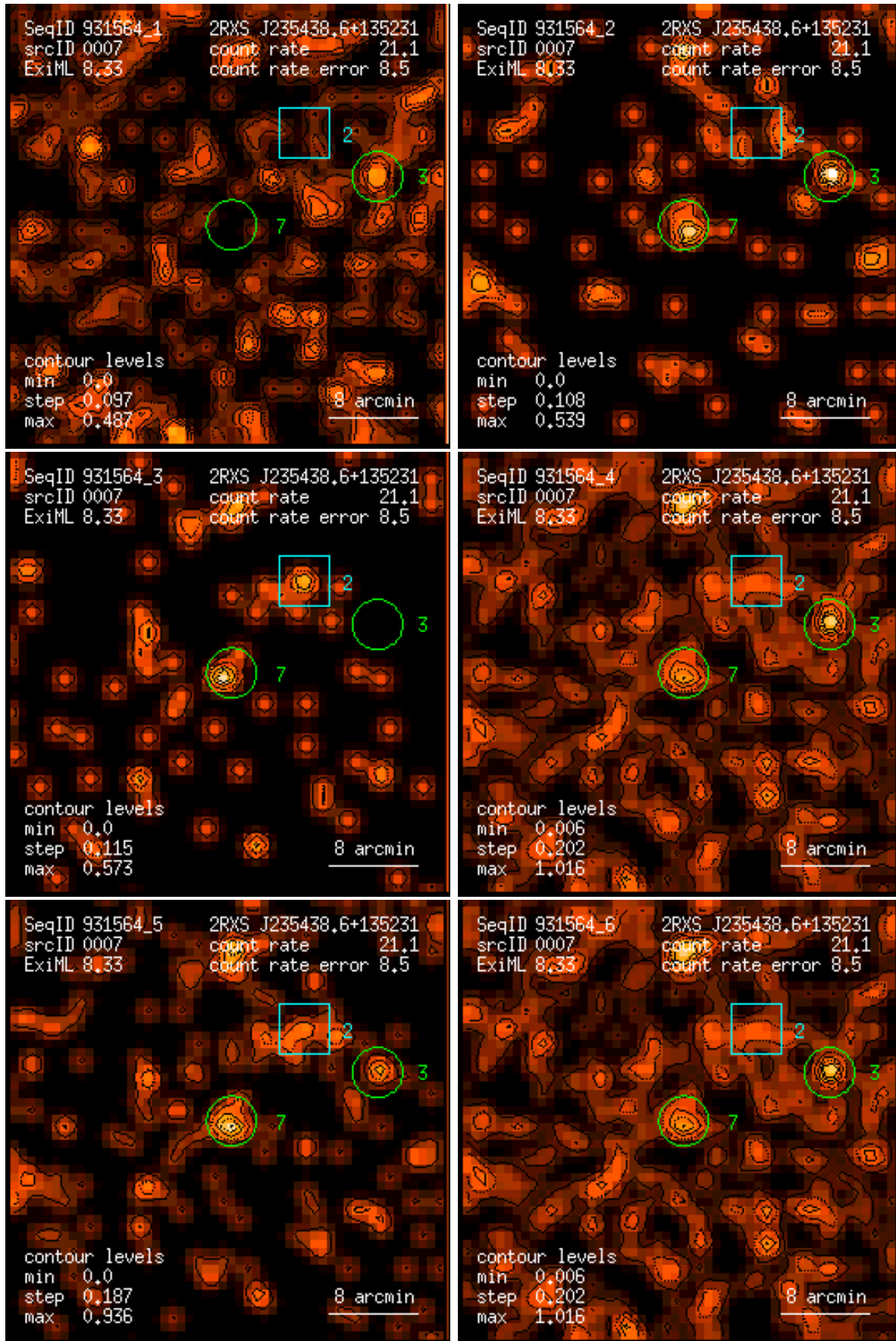
Figure 7: RASS 931564: detection 0007: band rate images, Gaussian filter: (1) PSPC channels 11 – 41, (2) 52 – 90, (3) 91 – 201, (4) 11 – 235, (5) 52 – 201, (6) 11 – 201. Broad band rates in counts/ks. Band rate contour levels in counts/ks/arcmin 2 .
