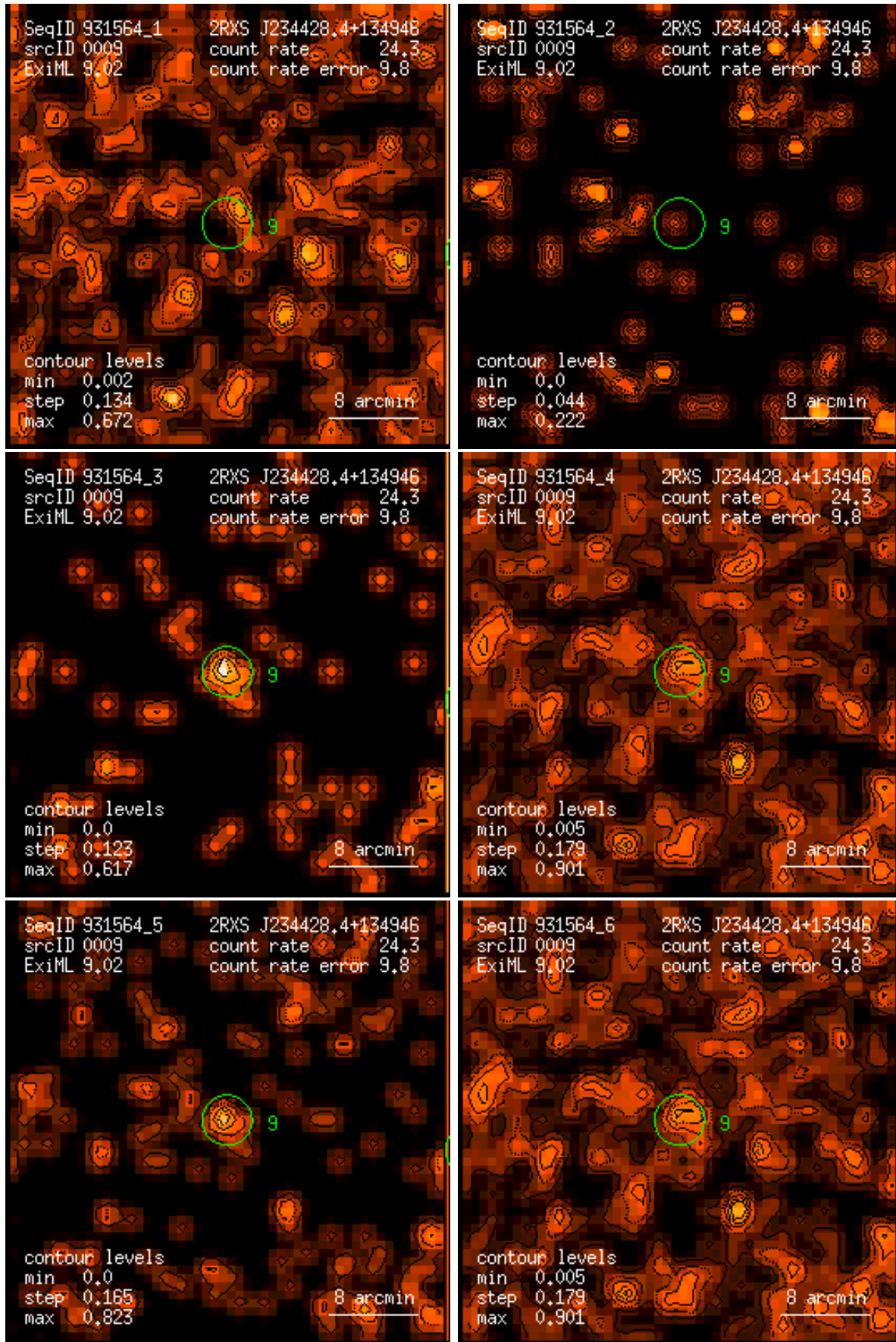
Figure 9: RASS 931564: detection 0009: band rate images, Gaussian filter: (1) PSPC channels 11 – 41, (2) 52 – 90, (3) 91 – 201, (4) 11 – 235, (5) 52 – 201, (6) 11 – 201. Broad band rates in counts/ks. Band rate contour levels in counts/ks/arcmin 2 .
