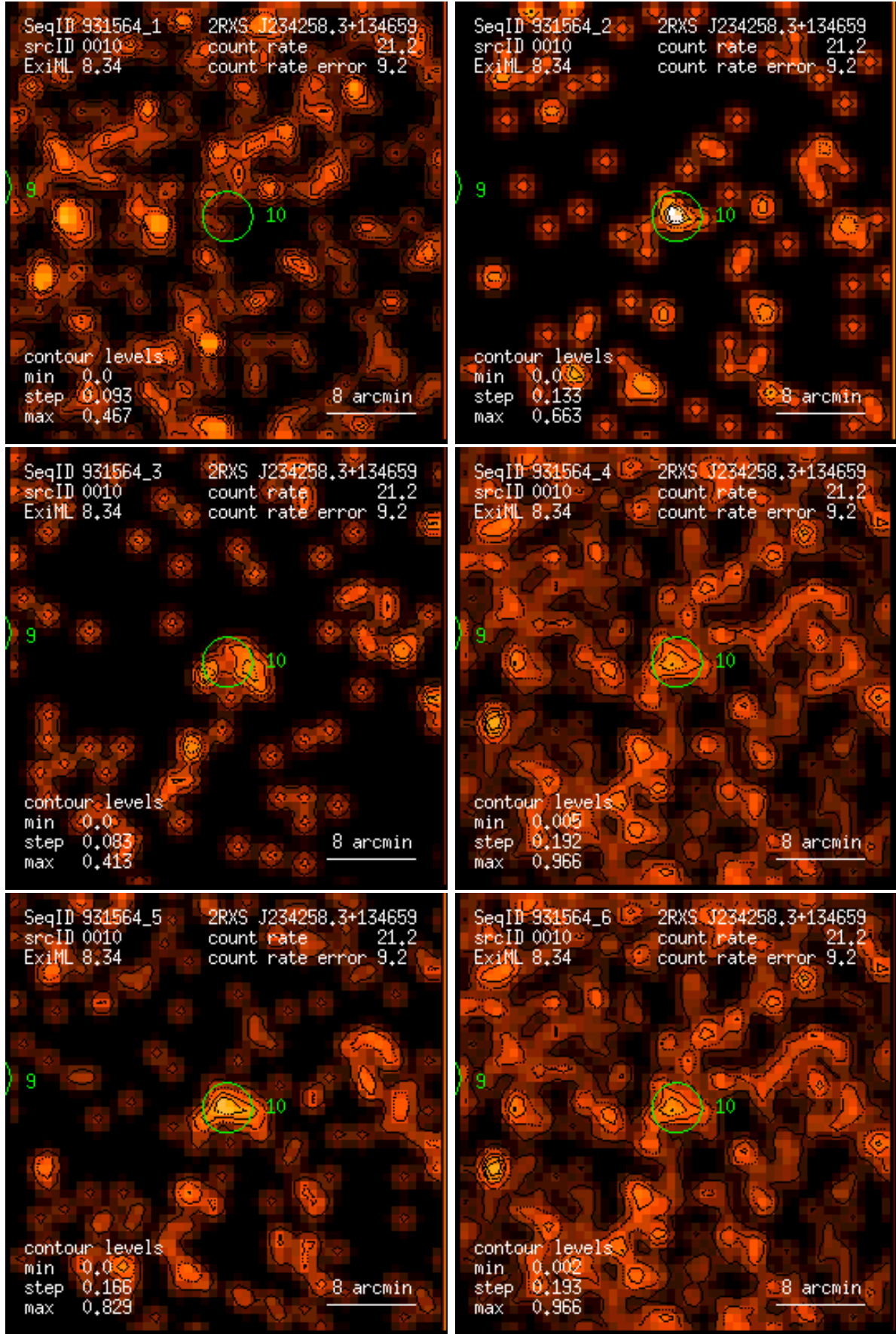
Figure 10: RASS 931564: detection 0010: band rate images, Gaussian filter: (1) PSPC channels 11 – 41, (2) 52 – 90, (3) 91 – 201, (4) 11 – 235, (5) 52 – 201, (6) 11 – 201. Broad band rates in counts/ks. Band rate contour levels in counts/ks/arcmin 2 .
