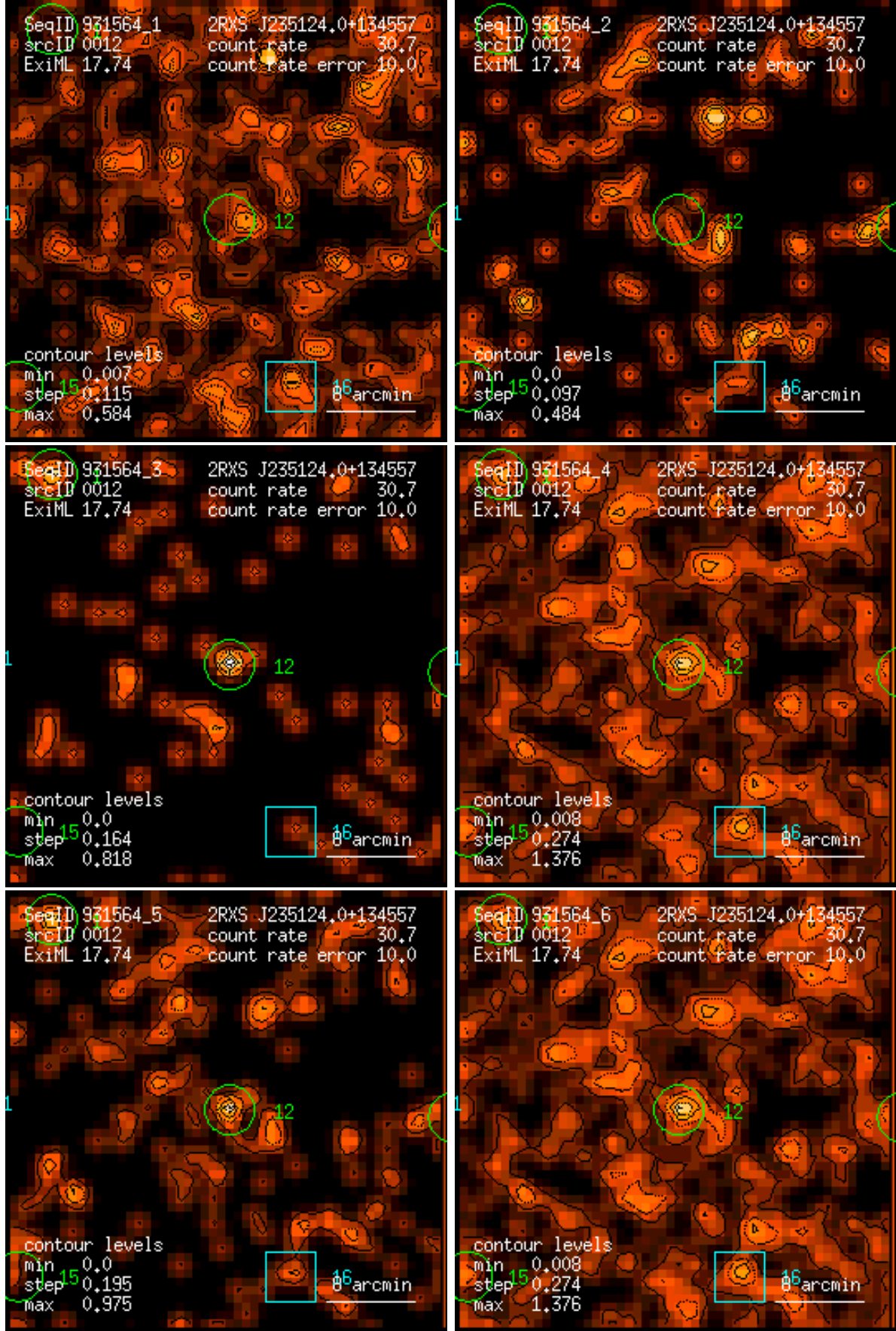
Figure 12: RASS 931564: detection 0012: band rate images, Gaussian filter: (1) PSPC channels 11 – 41, (2) 52 – 90, (3) 91 – 201, (4) 11 – 235, (5) 52 – 201, (6) 11 – 201. Broad band rates in counts/ks. Band rate contour levels in counts/ks/arcmin 2 .
