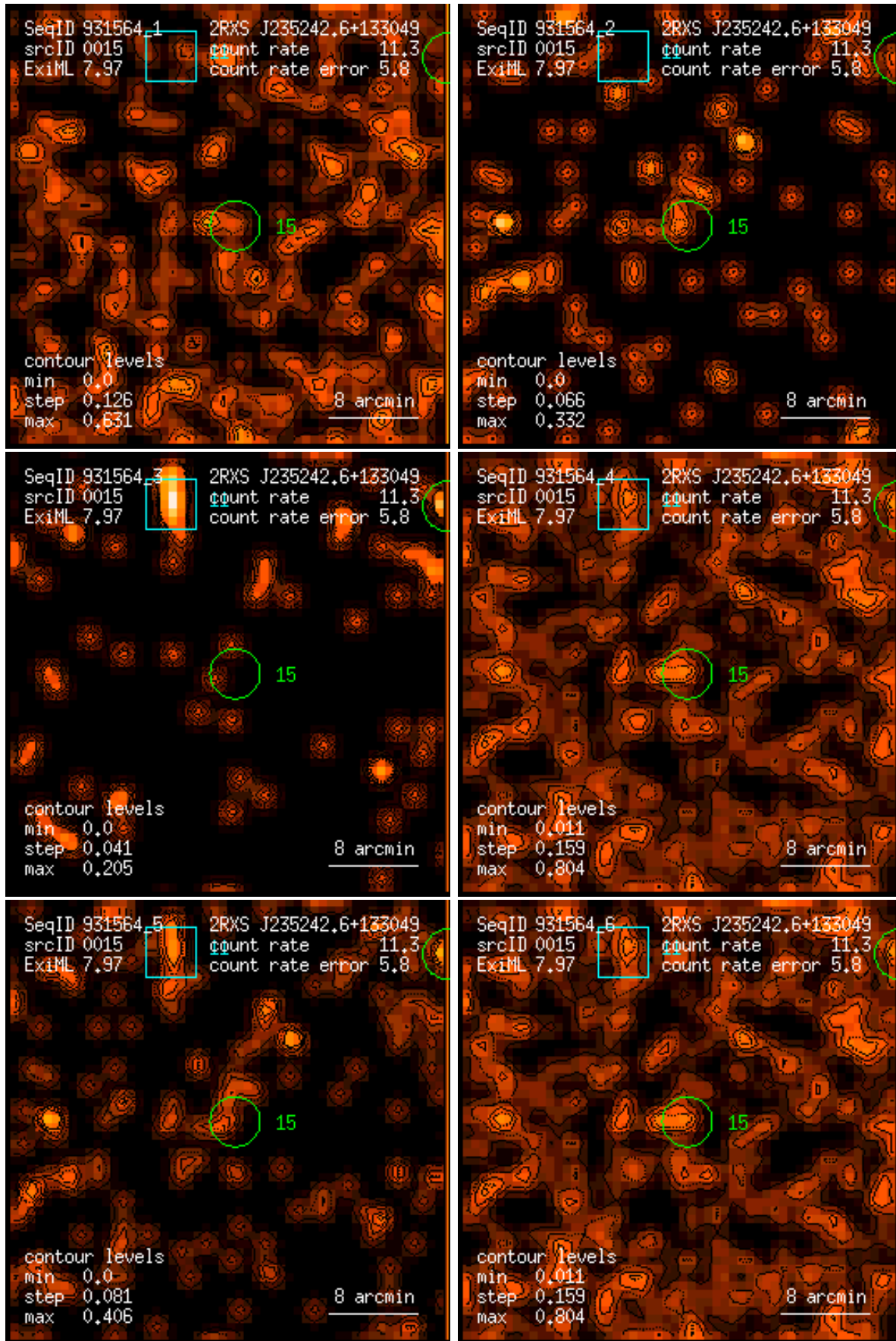
Figure 15: RASS 931564: detection 0015: band rate images, Gaussian filter: (1) PSPC channels 11 – 41, (2) 52 – 90, (3) 91 – 201, (4) 11 – 235, (5) 52 – 201, (6) 11 – 201. Broad band rates in counts/ks. Band rate contour levels in counts/ks/arcmin 2 .
