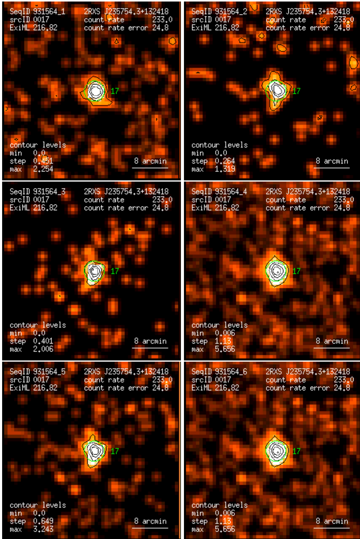
Figure 17: RASS 931564: detection 0017: band rate images, Gaussian filter: (1) PSPC channels 11 – 41, (2) 52 – 90, (3) 91 – 201, (4) 11 – 235, (5) 52 – 201, (6) 11 – 201. Broad band rates in counts/ks. Band rate contour levels in counts/ks/arcmin 2 .
