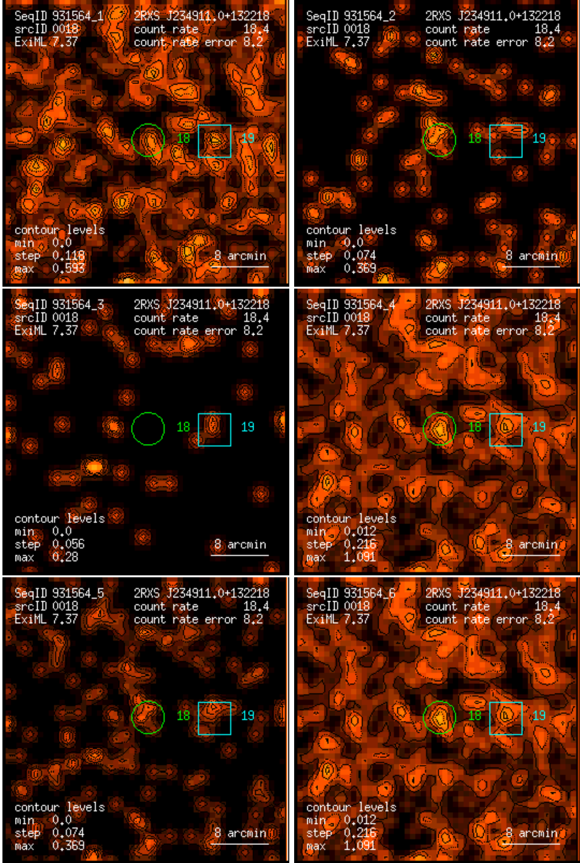
Figure 18: RASS 931564: detection 0018: band rate images, Gaussian filter: (1) PSPC channels 11 – 41, (2) 52 – 90, (3) 91 – 201, (4) 11 – 235, (5) 52 – 201, (6) 11 – 201. Broad band rates in counts/ks. Band rate contour levels in counts/ks/arcmin 2 .
