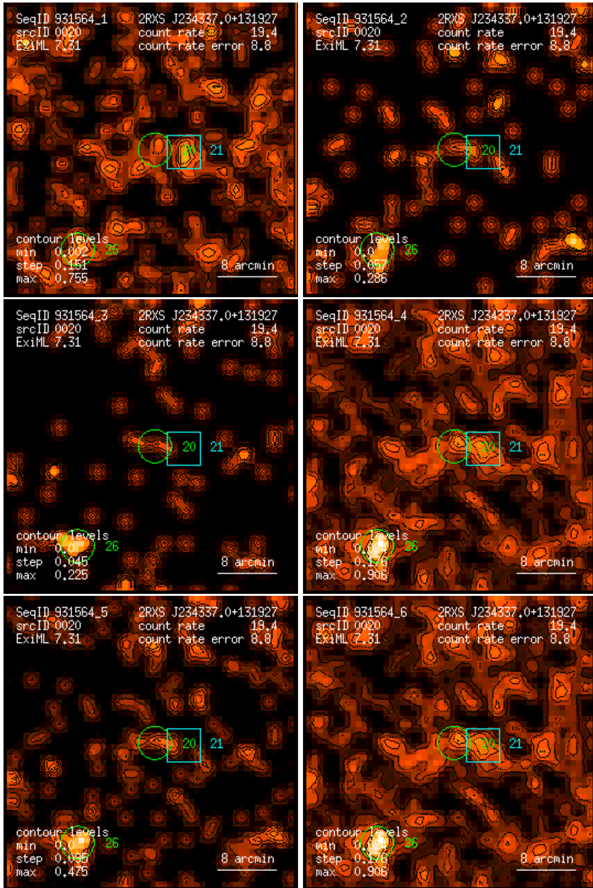
Figure 20: RASS 931564: detection 0020: band rate images, Gaussian filter: (1) PSPC channels 11 – 41, (2) 52 – 90, (3) 91 – 201, (4) 11 – 235, (5) 52 – 201, (6) 11 – 201. Broad band rates in counts/ks. Band rate contour levels in counts/ks/arcmin 2 .
