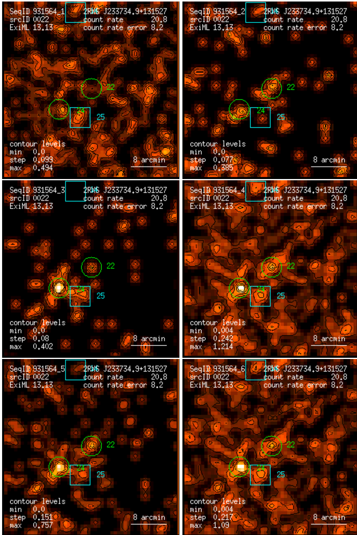
Figure 22: RASS 931564: detection 0022: band rate images, Gaussian filter: (1) PSPC channels 11 – 41, (2) 52 – 90, (3) 91 – 201, (4) 11 – 235, (5) 52 – 201, (6) 11 – 201. Broad band rates in counts/ks. Band rate contour levels in counts/ks/arcmin 2 .
