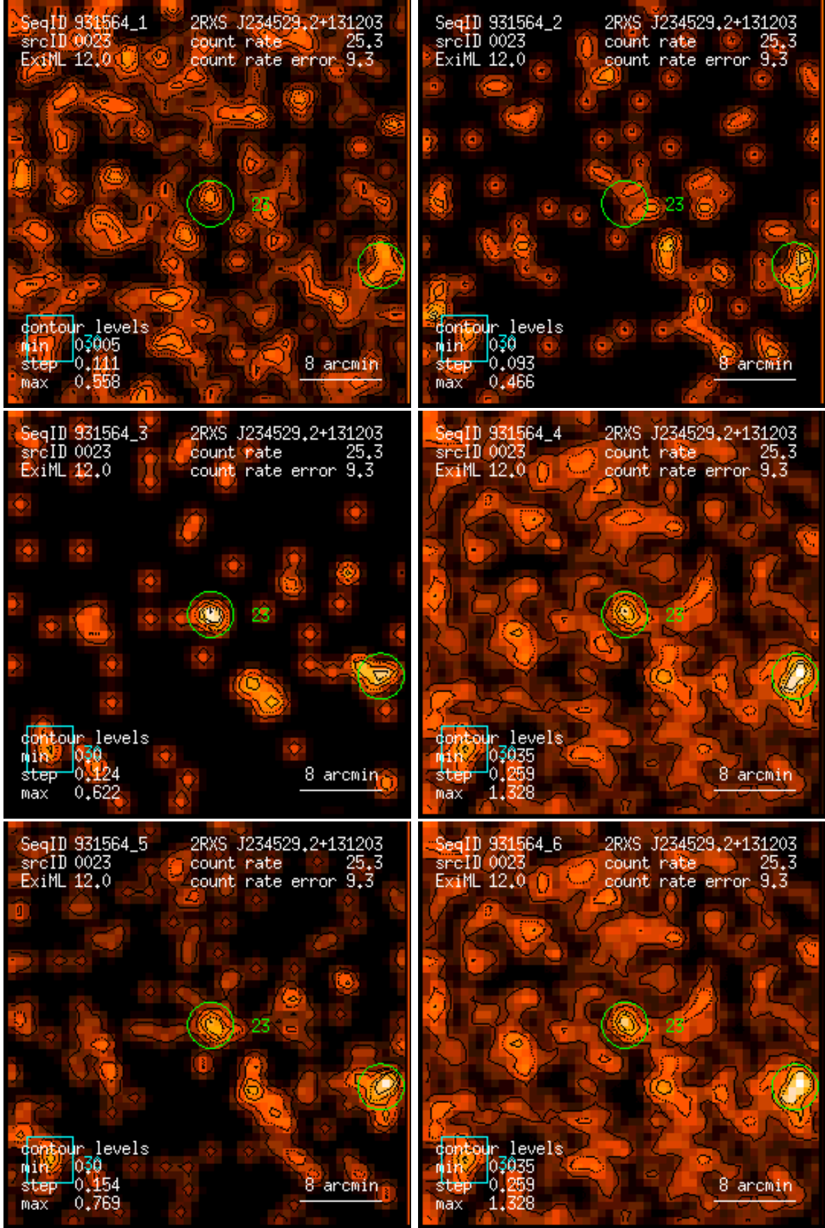
Figure 23: RASS 931564: detection 0023: band rate images, Gaussian filter: (1) PSPC channels 11 – 41, (2) 52 – 90, (3) 91 – 201, (4) 11 – 235, (5) 52 – 201, (6) 11 – 201. Broad band rates in counts/ks. Band rate contour levels in counts/ks/arcmin 2 .
